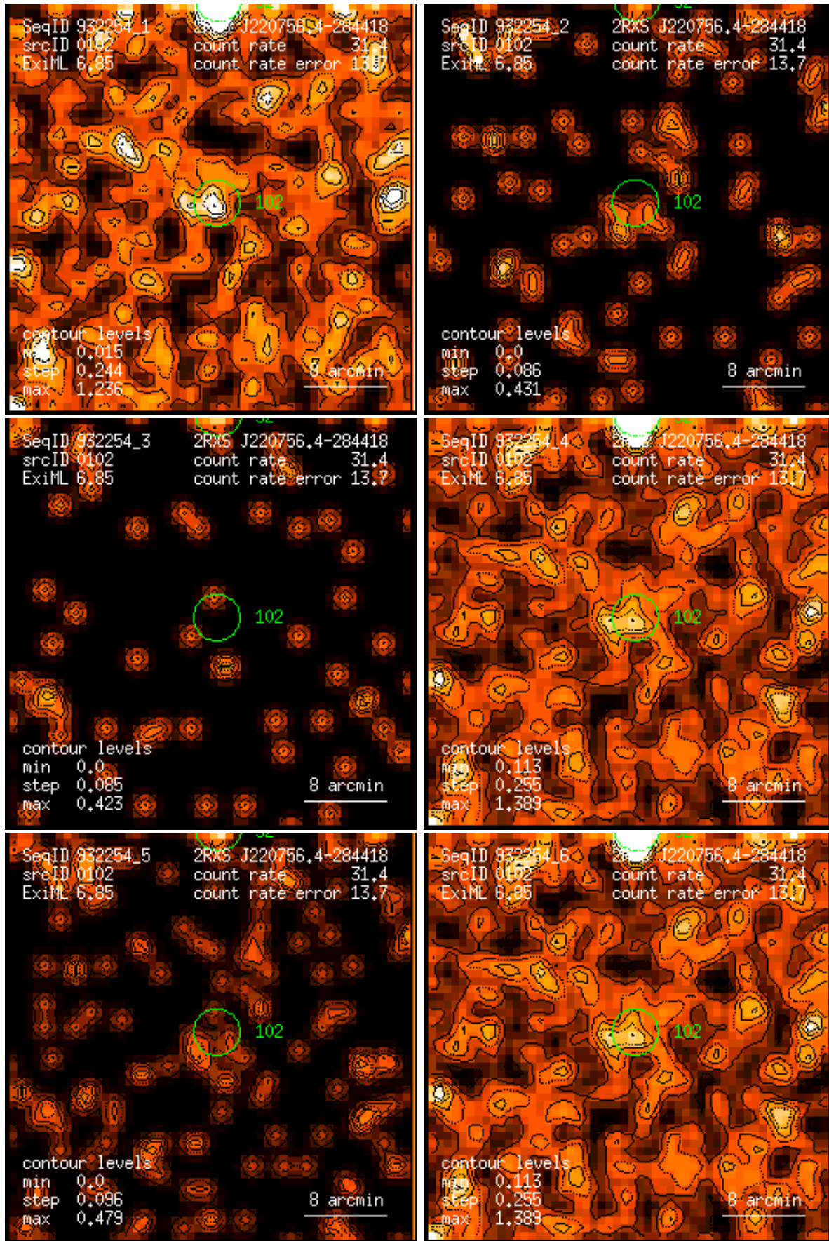
Figure 102: RASS 932254: detection 0102: band rate images, Gaussian filter: (1) PSPC channels 11 – 41, (2) 52 – 90, (3) 91 – 201, (4) 11 – 235, (5) 52 – 201, (6) 11 – 201. Broad band rates in counts/ks. Band rate contour levels in counts/ks/arcmin 2 .
