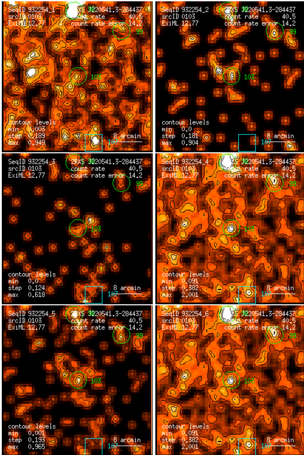
Figure 103: RASS 932254: detection 0103: band rate images, Gaussian filter: (1) PSPC channels 11 – 41, (2) 52 – 90, (3) 91 – 201, (4) 11 – 235, (5) 52 – 201, (6) 11 – 201. Broad band rates in counts/ks. Band rate contour levels in counts/ks/arcmin 2 .
