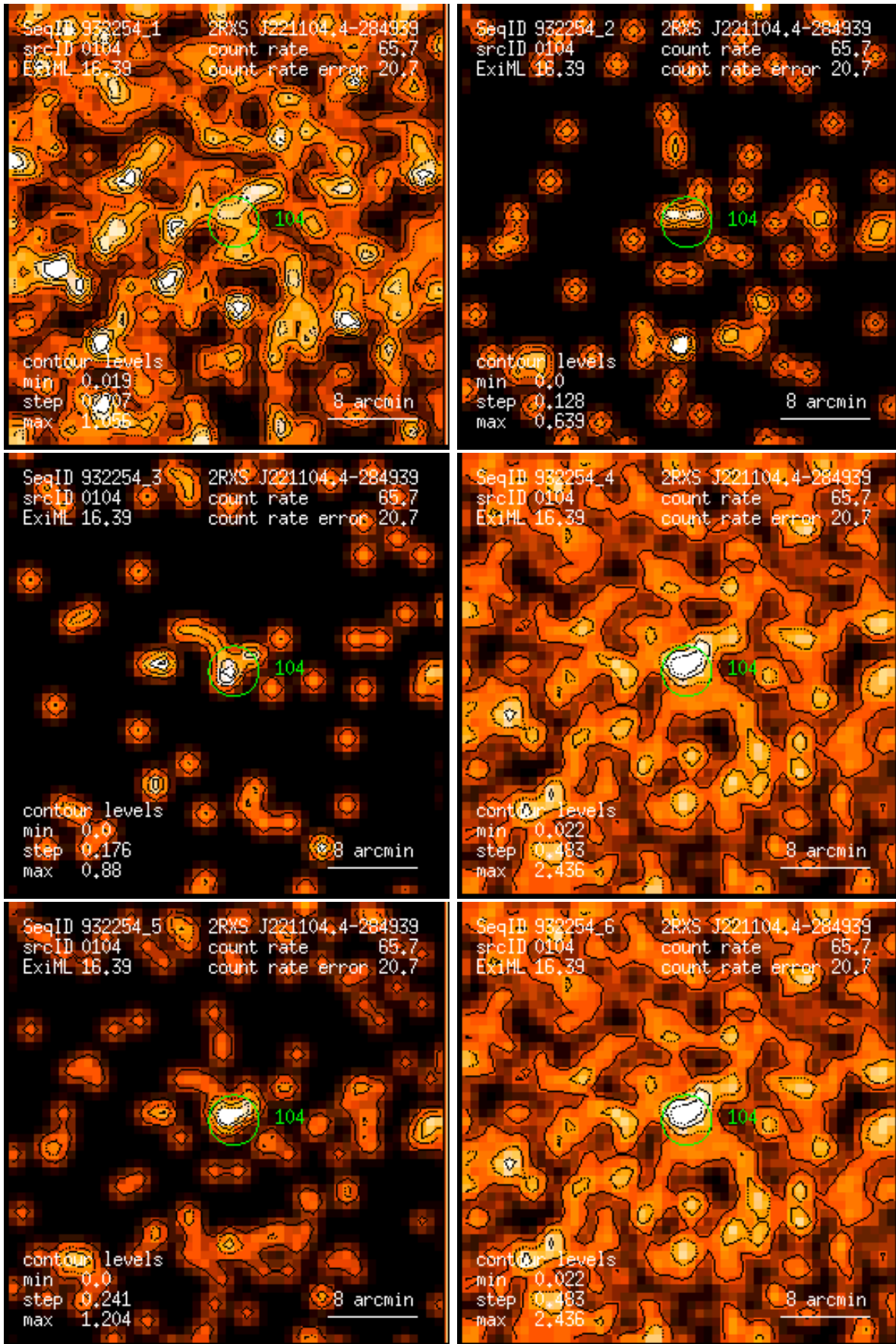
Figure 104: RASS 932254: detection 0104: band rate images, Gaussian filter: (1) PSPC channels 11 – 41, (2) 52 – 90, (3) 91 – 201, (4) 11 – 235, (5) 52 – 201, (6) 11 – 201. Broad band rates in counts/ks. Band rate contour levels in counts/ks/arcmin 2 .
