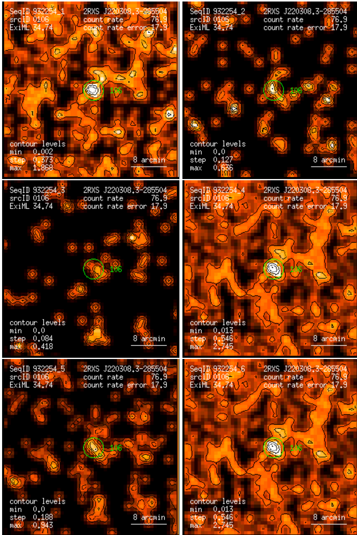
Figure 106: RASS 932254: detection 0106: band rate images, Gaussian filter: (1) PSPC channels 11 – 41, (2) 52 – 90, (3) 91 – 201, (4) 11 – 235, (5) 52 – 201, (6) 11 – 201. Broad band rates in counts/ks. Band rate contour levels in counts/ks/arcmin 2 .
