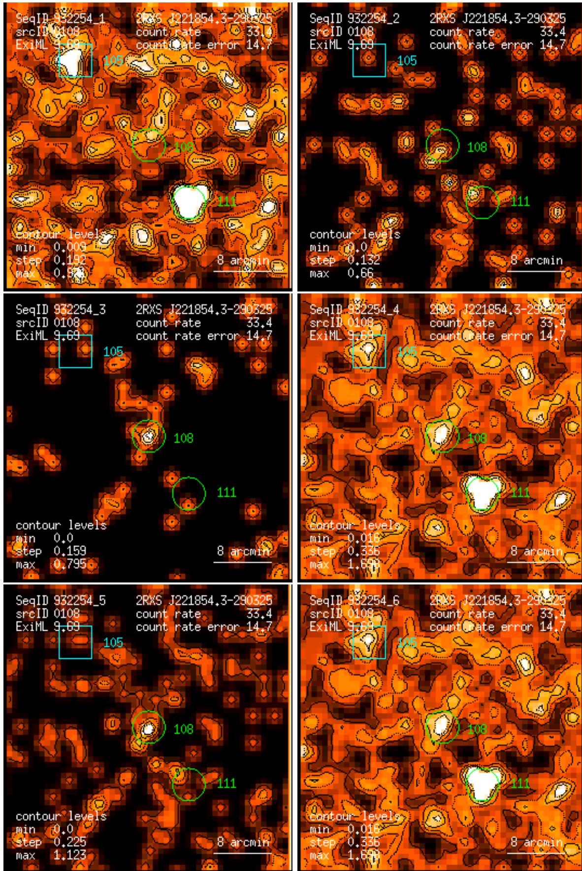
Figure 108: RASS 932254: detection 0108: band rate images, Gaussian filter: (1) PSPC channels 11 – 41, (2) 52 – 90, (3) 91 – 201, (4) 11 – 235, (5) 52 – 201, (6) 11 – 201. Broad band rates in counts/ks. Band rate contour levels in counts/ks/arcmin 2 .
