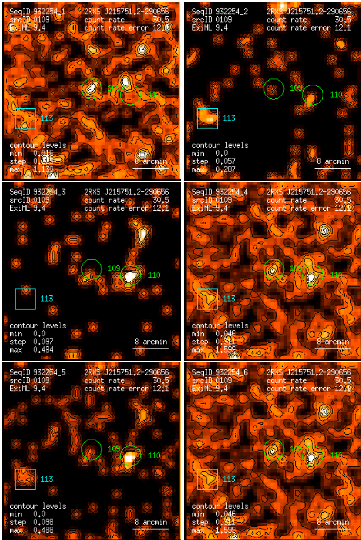
Figure 109: RASS 932254: detection 0109: band rate images, Gaussian filter: (1) PSPC channels 11 – 41, (2) 52 – 90, (3) 91 – 201, (4) 11 – 235, (5) 52 – 201, (6) 11 – 201. Broad band rates in counts/ks. Band rate contour levels in counts/ks/arcmin 2 .
