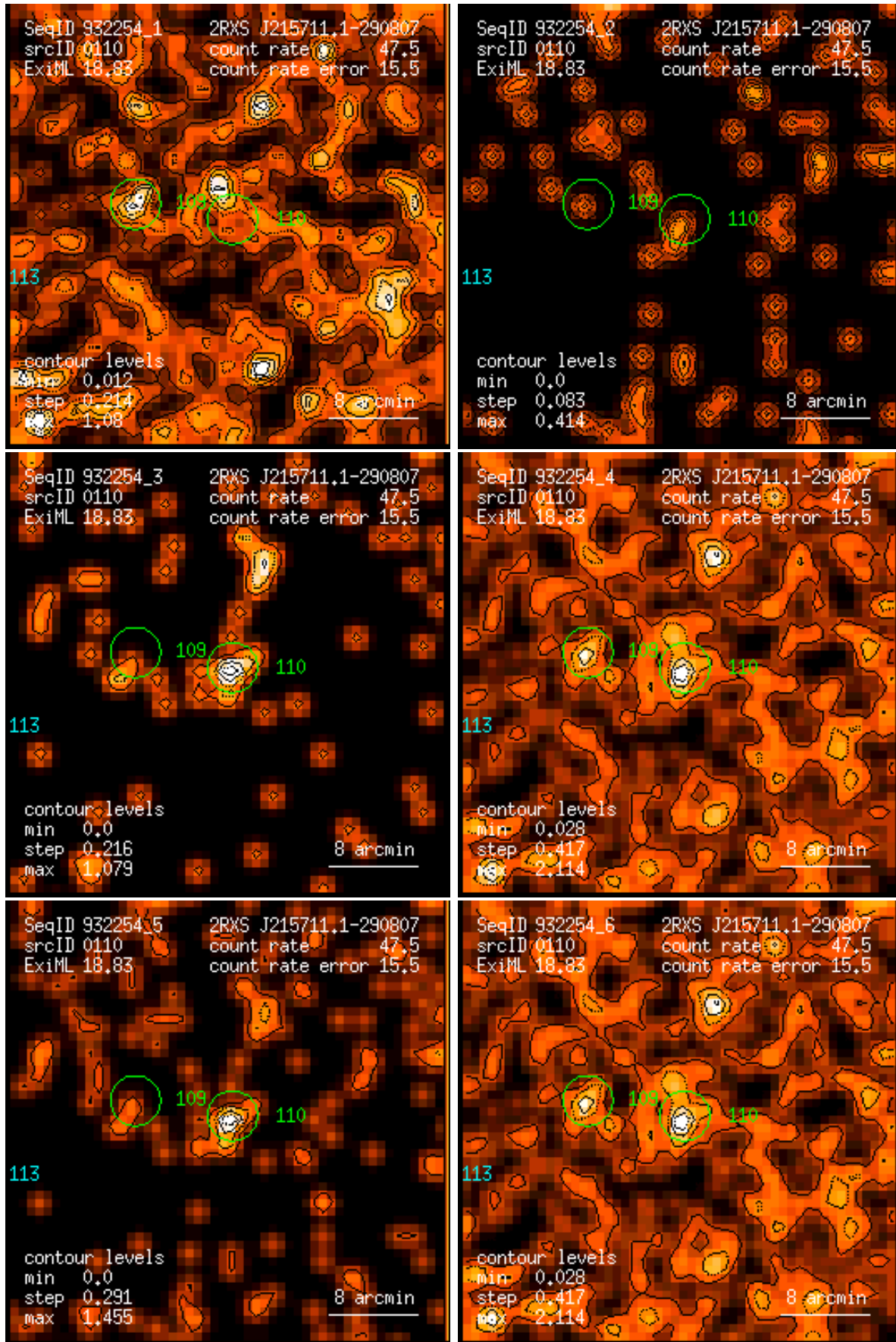
Figure 110: RASS 932254: detection 0110: band rate images, Gaussian filter: (1) PSPC channels 11 – 41, (2) 52 – 90, (3) 91 – 201, (4) 11 – 235, (5) 52 – 201, (6) 11 – 201. Broad band rates in counts/ks. Band rate contour levels in counts/ks/arcmin 2 .
