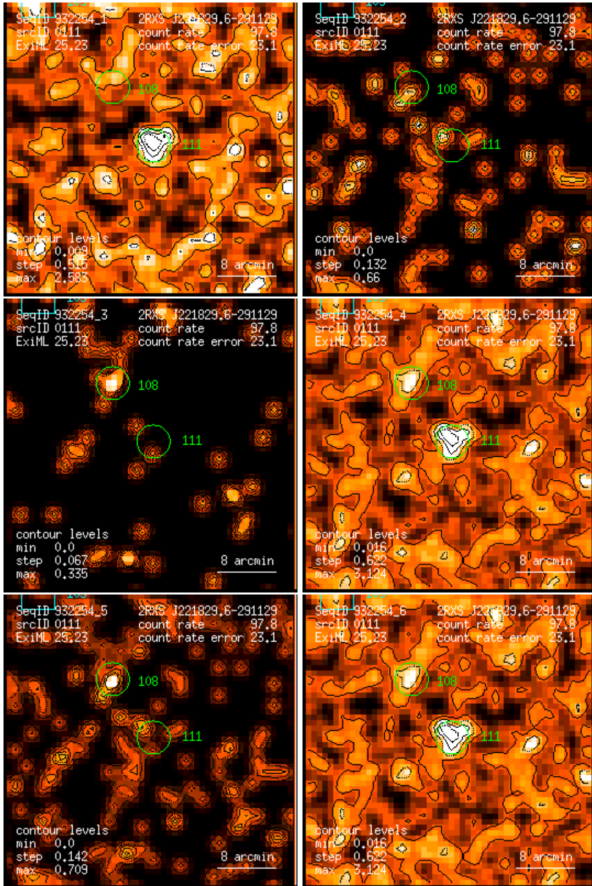
Figure 111: RASS 932254: detection 0111: band rate images, Gaussian filter: (1) PSPC channels 11 – 41, (2) 52 – 90, (3) 91 – 201, (4) 11 – 235, (5) 52 – 201, (6) 11 – 201. Broad band rates in counts/ks. Band rate contour levels in counts/ks/arcmin 2 .
