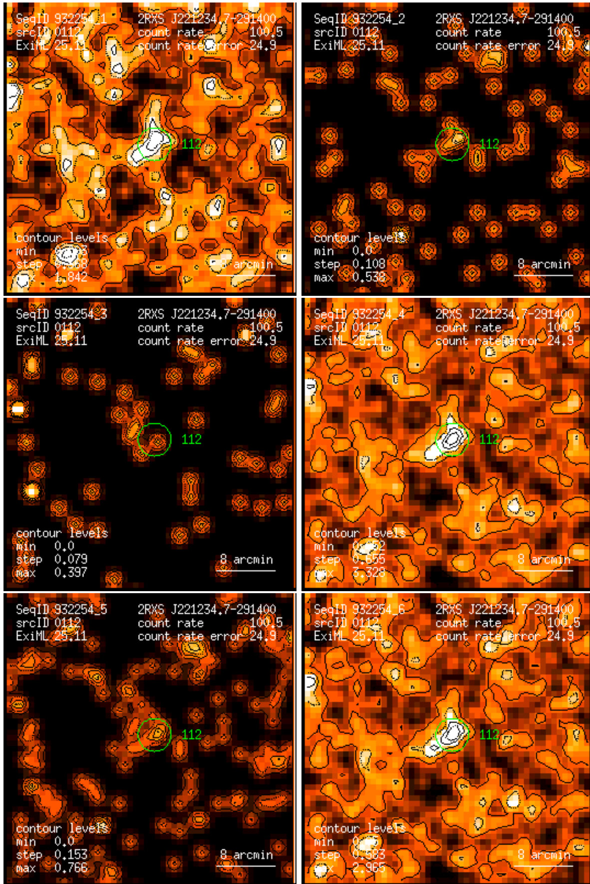
Figure 112: RASS 932254: detection 0112: band rate images, Gaussian filter: (1) PSPC channels 11 – 41, (2) 52 – 90, (3) 91 – 201, (4) 11 – 235, (5) 52 – 201, (6) 11 – 201. Broad band rates in counts/ks. Band rate contour levels in counts/ks/arcmin 2 .
