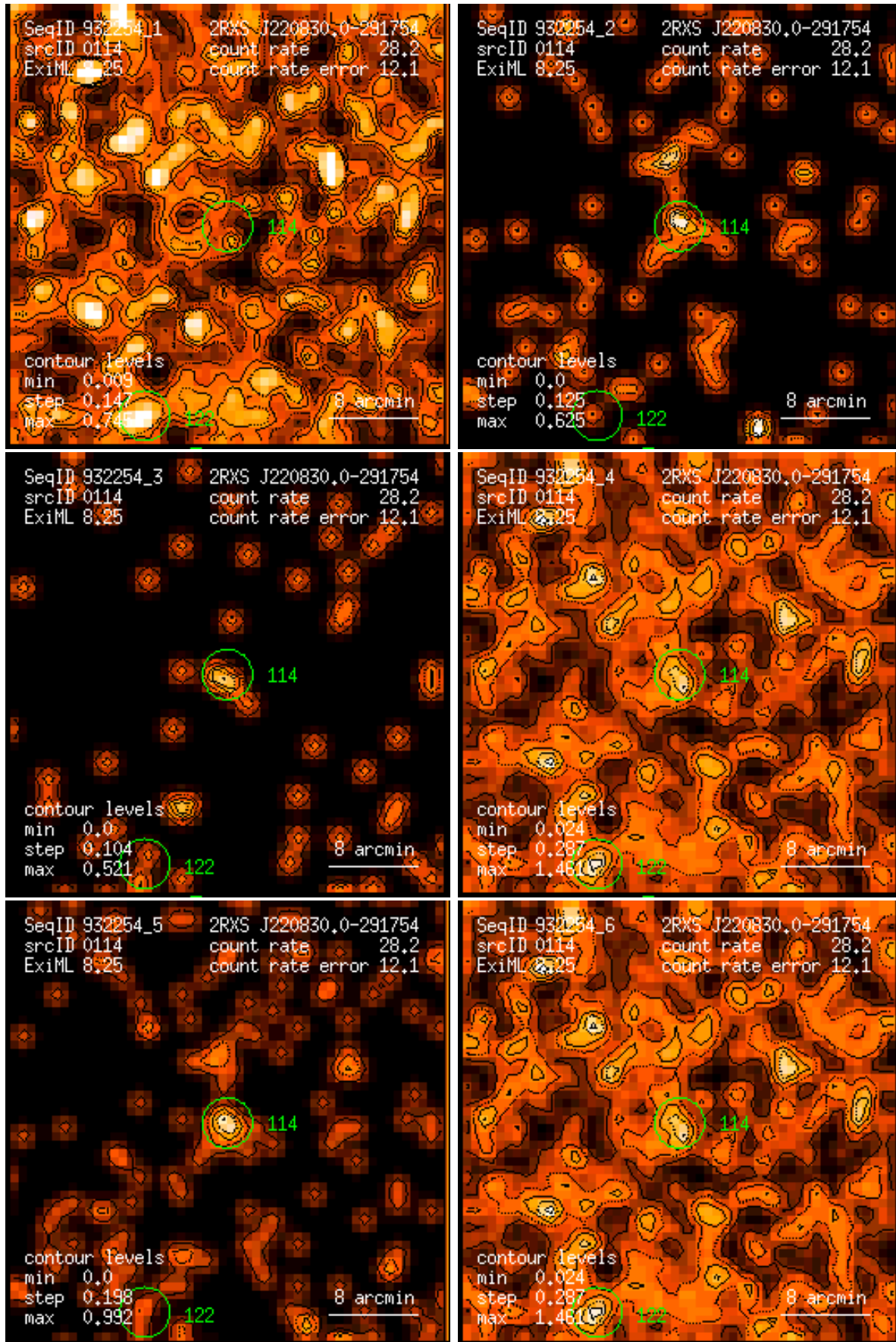
Figure 114: RASS 932254: detection 0114: band rate images, Gaussian filter: (1) PSPC channels 11 – 41, (2) 52 – 90, (3) 91 – 201, (4) 11 – 235, (5) 52 – 201, (6) 11 – 201. Broad band rates in counts/ks. Band rate contour levels in counts/ks/arcmin 2 .
