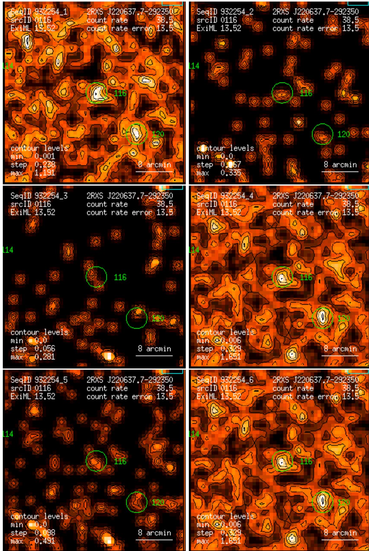
Figure 116: RASS 932254: detection 0116: band rate images, Gaussian filter: (1) PSPC channels 11 – 41, (2) 52 – 90, (3) 91 – 201, (4) 11 – 235, (5) 52 – 201, (6) 11 – 201. Broad band rates in counts/ks. Band rate contour levels in counts/ks/arcmin 2 .
