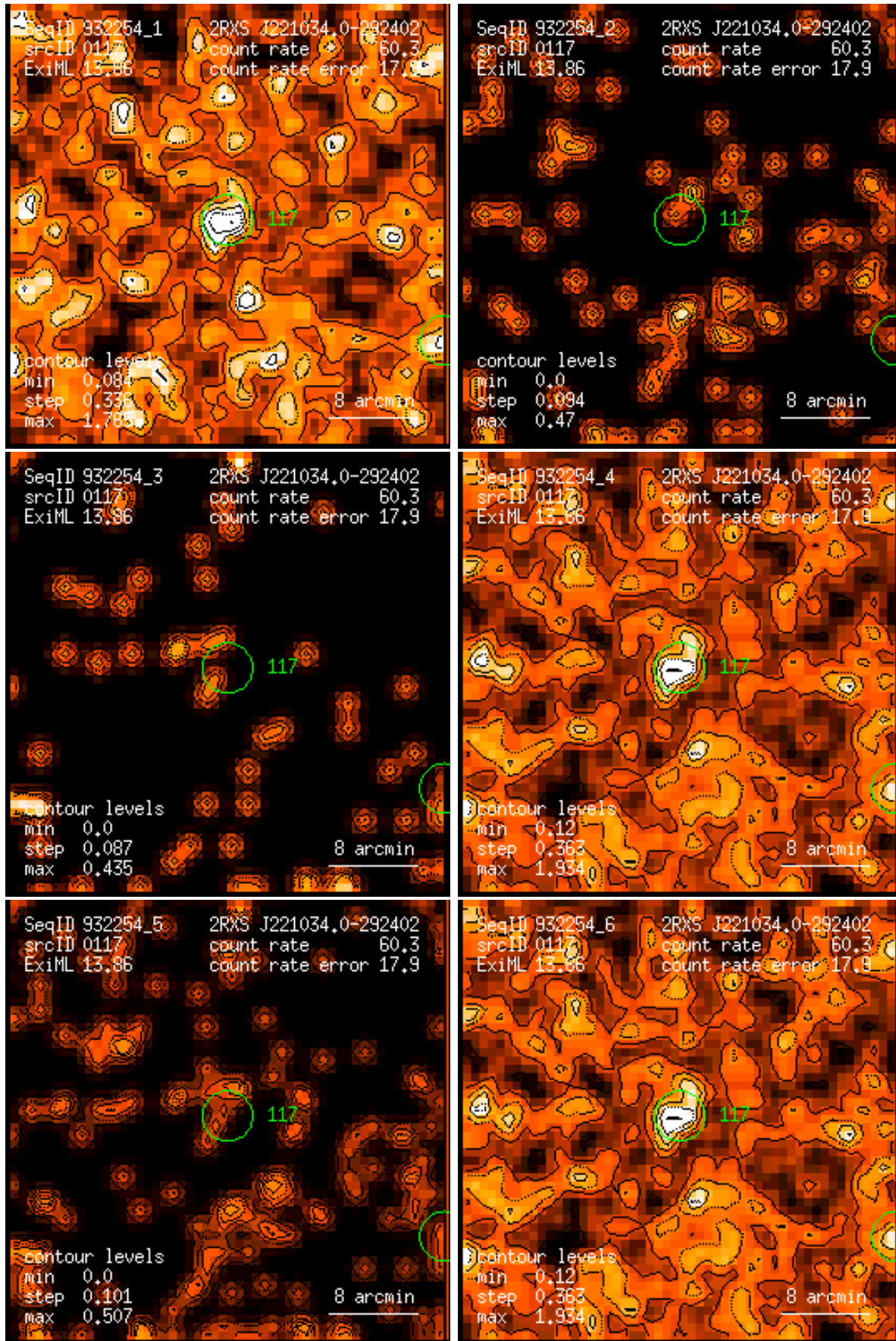
Figure 117: RASS 932254: detection 0117: band rate images, Gaussian filter: (1) PSPC channels 11 – 41, (2) 52 – 90, (3) 91 – 201, (4) 11 – 235, (5) 52 – 201, (6) 11 – 201. Broad band rates in counts/ks. Band rate contour levels in counts/ks/arcmin 2 .
