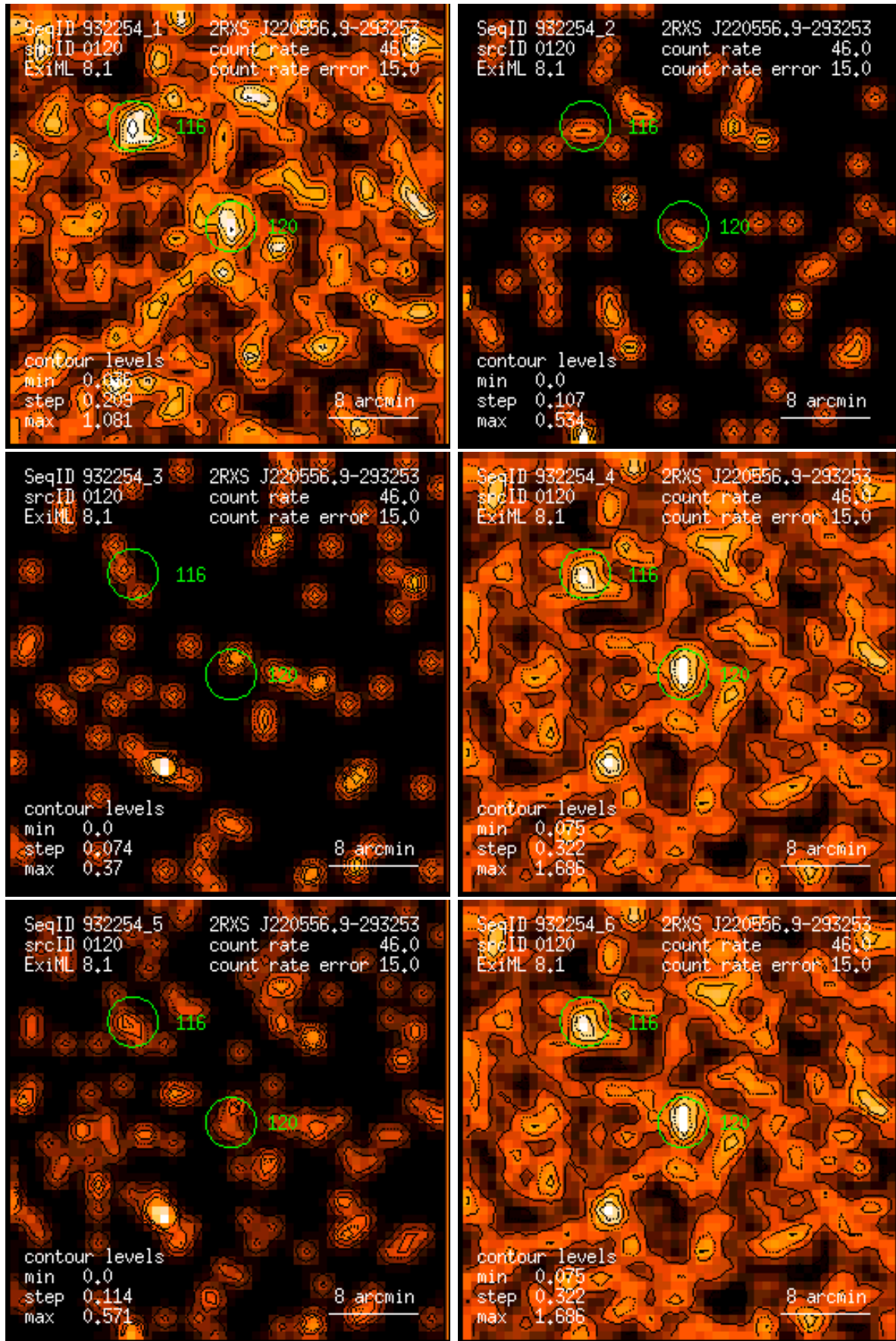
Figure 120: RASS 932254: detection 0120: band rate images, Gaussian filter: (1) PSPC channels 11 – 41, (2) 52 – 90, (3) 91 – 201, (4) 11 – 235, (5) 52 – 201, (6) 11 – 201. Broad band rates in counts/ks. Band rate contour levels in counts/ks/arcmin 2 .
