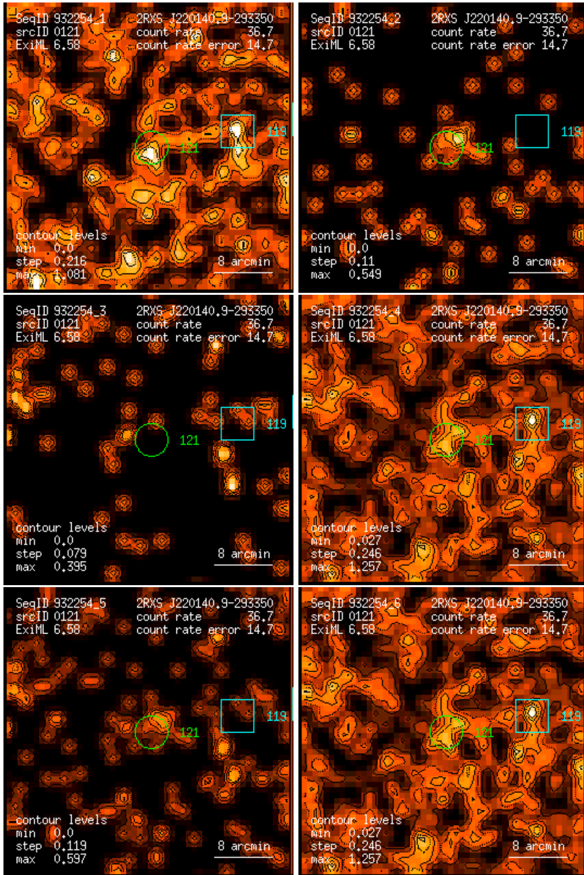
Figure 121: RASS 932254: detection 0121: band rate images, Gaussian filter: (1) PSPC channels 11 – 41, (2) 52 – 90, (3) 91 – 201, (4) 11 – 235, (5) 52 – 201, (6) 11 – 201. Broad band rates in counts/ks. Band rate contour levels in counts/ks/arcmin 2 .
