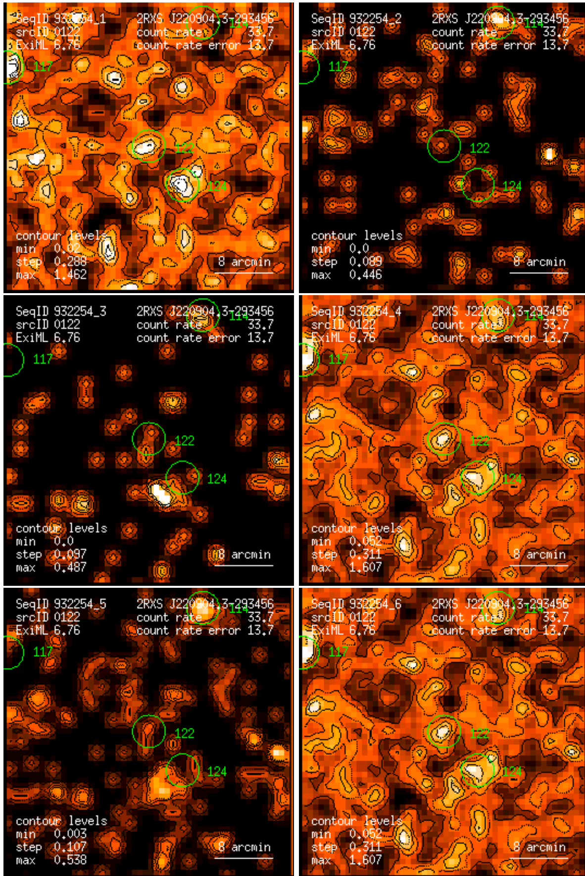
Figure 122: RASS 932254: detection 0122: band rate images, Gaussian filter: (1) PSPC channels 11 – 41, (2) 52 – 90, (3) 91 – 201, (4) 11 – 235, (5) 52 – 201, (6) 11 – 201. Broad band rates in counts/ks. Band rate contour levels in counts/ks/arcmin 2 .
