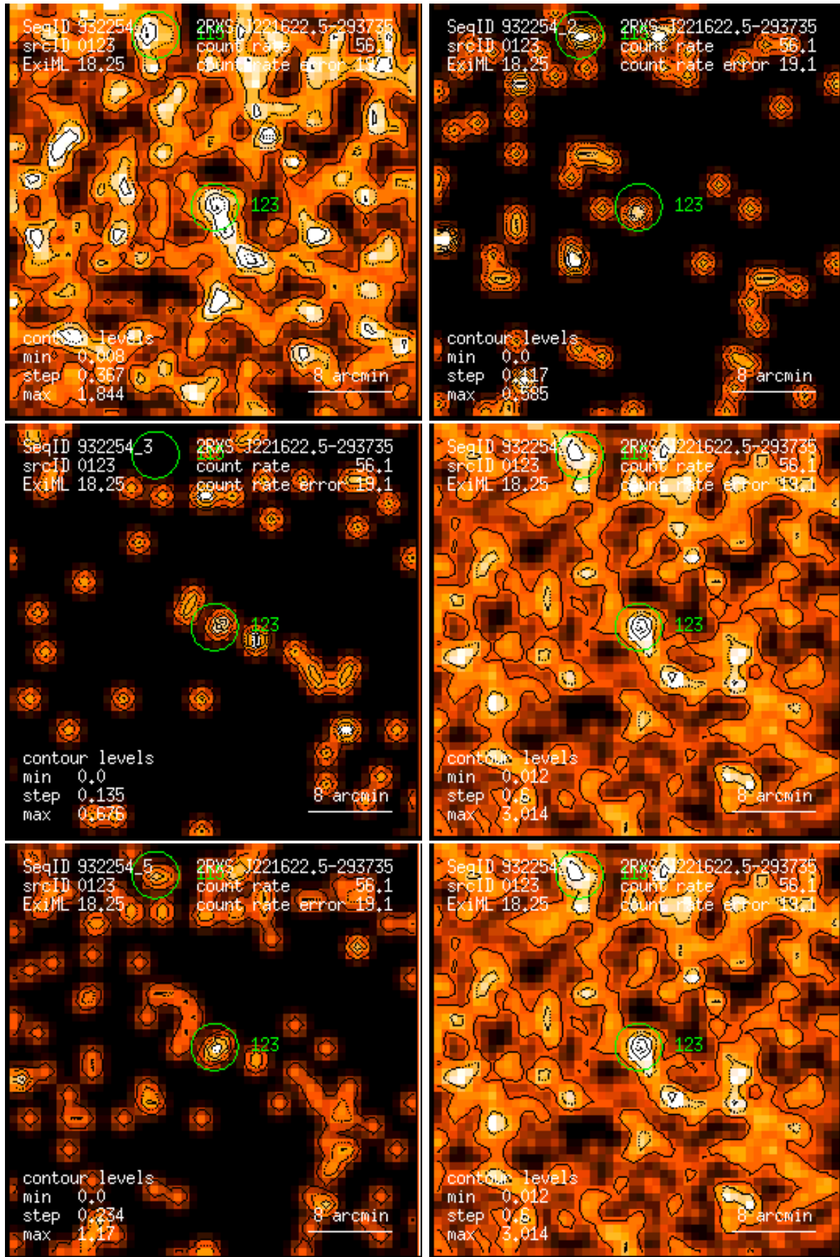
Figure 123: RASS 932254: detection 0123: band rate images, Gaussian filter: (1) PSPC channels 11 – 41, (2) 52 – 90, (3) 91 – 201, (4) 11 – 235, (5) 52 – 201, (6) 11 – 201. Broad band rates in counts/ks. Band rate contour levels in counts/ks/arcmin 2 .
