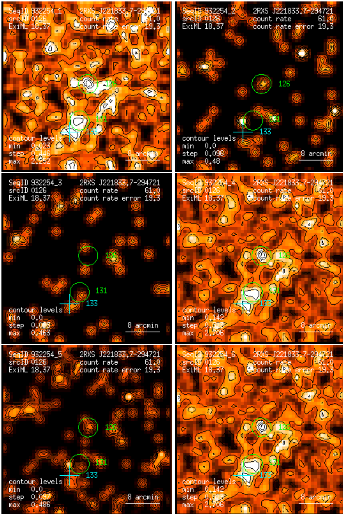
Figure 126: RASS 932254: detection 0126: band rate images, Gaussian filter: (1) PSPC channels 11 – 41, (2) 52 – 90, (3) 91 – 201, (4) 11 – 235, (5) 52 – 201, (6) 11 – 201. Broad band rates in counts/ks. Band rate contour levels in counts/ks/arcmin 2 .
