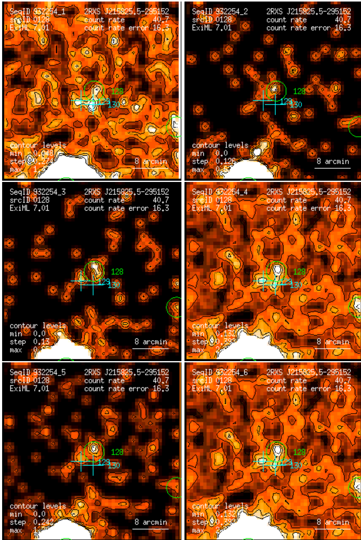
Figure 128: RASS 932254: detection 0128: band rate images, Gaussian filter: (1) PSPC channels 11 – 41, (2) 52 – 90, (3) 91 – 201, (4) 11 – 235, (5) 52 – 201, (6) 11 – 201. Broad band rates in counts/ks. Band rate contour levels in counts/ks/arcmin 2 .
