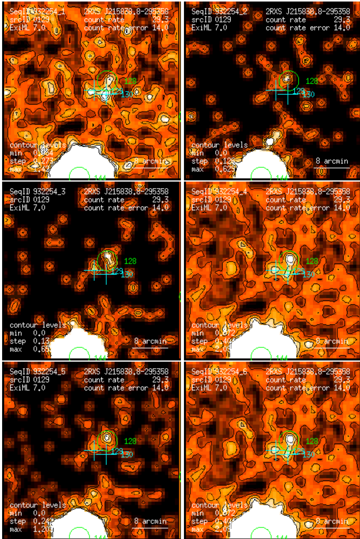
Figure 129: RASS 932254: detection 0129: band rate images, Gaussian filter: (1) PSPC channels 11 – 41, (2) 52 – 90, (3) 91 – 201, (4) 11 – 235, (5) 52 – 201, (6) 11 – 201. Broad band rates in counts/ks. Band rate contour levels in counts/ks/arcmin 2 .
