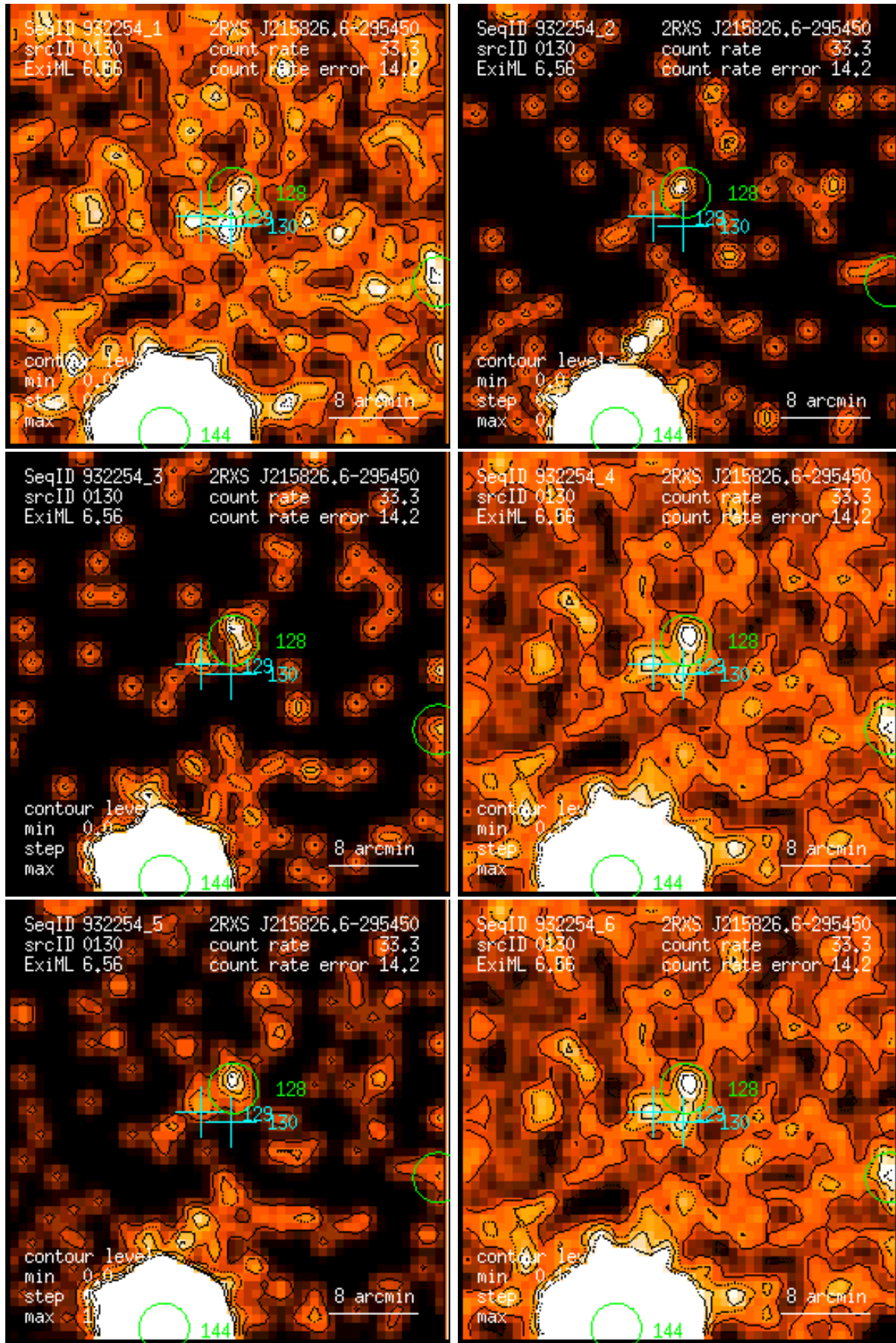
Figure 130: RASS 932254: detection 0130: band rate images, Gaussian filter: (1) PSPC channels 11 – 41, (2) 52 – 90, (3) 91 – 201, (4) 11 – 235, (5) 52 – 201, (6) 11 – 201. Broad band rates in counts/ks. Band rate contour levels in counts/ks/arcmin 2 .
