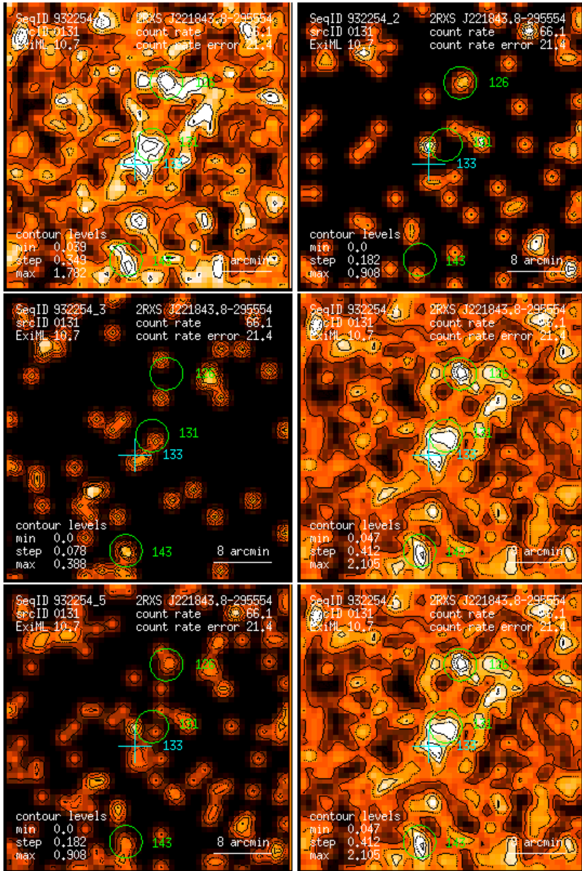
Figure 131: RASS 932254: detection 0131: band rate images, Gaussian filter: (1) PSPC channels 11 – 41, (2) 52 – 90, (3) 91 – 201, (4) 11 – 235, (5) 52 – 201, (6) 11 – 201. Broad band rates in counts/ks. Band rate contour levels in counts/ks/arcmin 2 .
