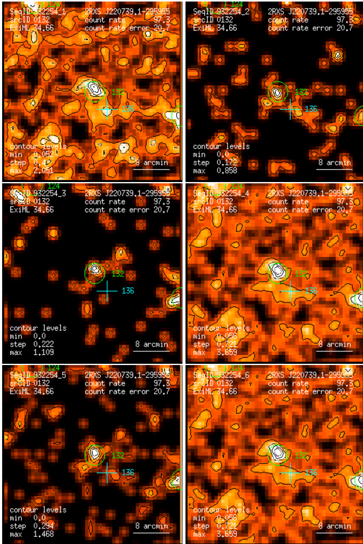
Figure 132: RASS 932254: detection 0132: band rate images, Gaussian filter: (1) PSPC channels 11 – 41, (2) 52 – 90, (3) 91 – 201, (4) 11 – 235, (5) 52 – 201, (6) 11 – 201. Broad band rates in counts/ks. Band rate contour levels in counts/ks/arcmin 2 .
