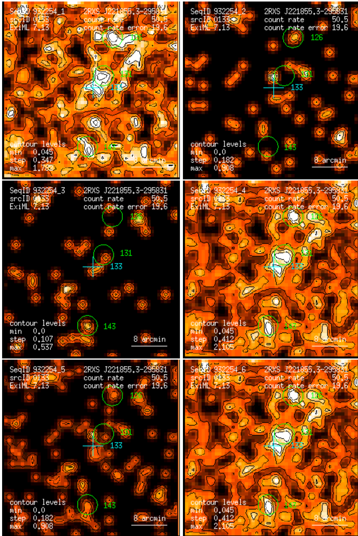
Figure 133: RASS 932254: detection 0133: band rate images, Gaussian filter: (1) PSPC channels 11 – 41, (2) 52 – 90, (3) 91 – 201, (4) 11 – 235, (5) 52 – 201, (6) 11 – 201. Broad band rates in counts/ks. Band rate contour levels in counts/ks/arcmin 2 .
