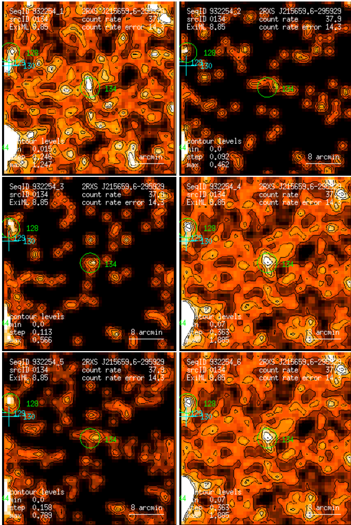
Figure 134: RASS 932254: detection 0134: band rate images, Gaussian filter: (1) PSPC channels 11 – 41, (2) 52 – 90, (3) 91 – 201, (4) 11 – 235, (5) 52 – 201, (6) 11 – 201. Broad band rates in counts/ks. Band rate contour levels in counts/ks/arcmin 2 .
