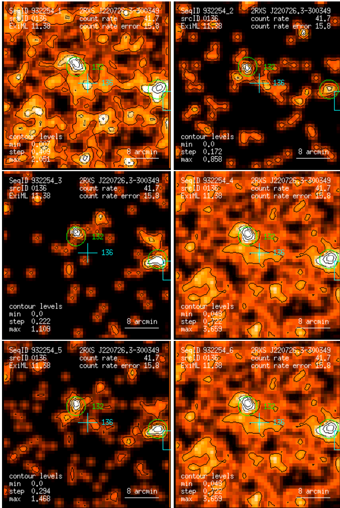
Figure 136: RASS 932254: detection 0136: band rate images, Gaussian filter: (1) PSPC channels 11 – 41, (2) 52 – 90, (3) 91 – 201, (4) 11 – 235, (5) 52 – 201, (6) 11 – 201. Broad band rates in counts/ks. Band rate contour levels in counts/ks/arcmin 2 .
