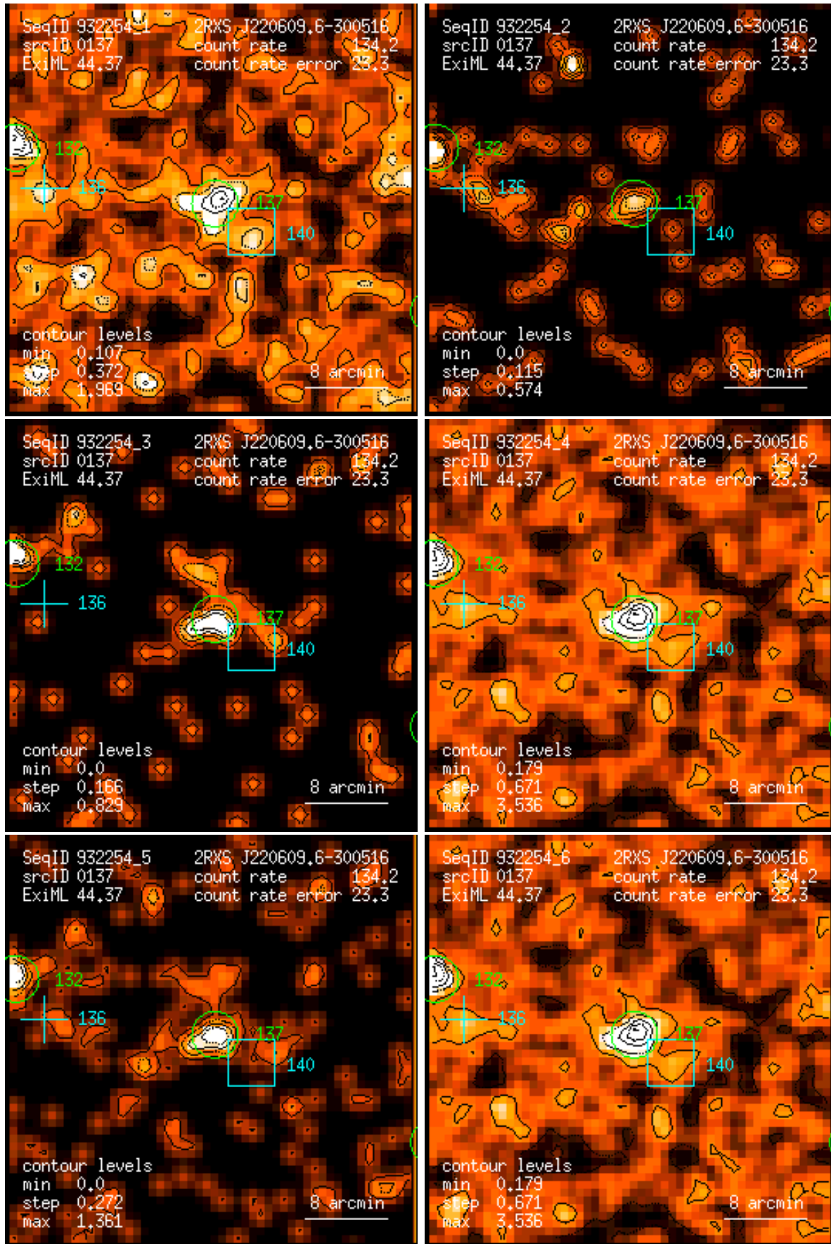
Figure 137: RASS 932254: detection 0137: band rate images, Gaussian filter: (1) PSPC channels 11 – 41, (2) 52 – 90, (3) 91 – 201, (4) 11 – 235, (5) 52 – 201, (6) 11 – 201. Broad band rates in counts/ks. Band rate contour levels in counts/ks/arcmin 2 .
