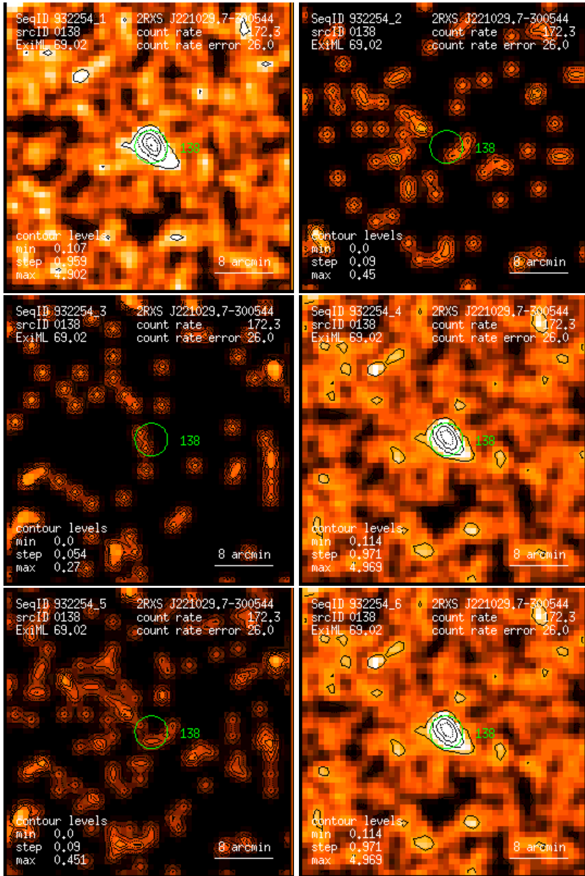
Figure 138: RASS 932254: detection 0138: band rate images, Gaussian filter: (1) PSPC channels 11 – 41, (2) 52 – 90, (3) 91 – 201, (4) 11 – 235, (5) 52 – 201, (6) 11 – 201. Broad band rates in counts/ks. Band rate contour levels in counts/ks/arcmin 2 .
