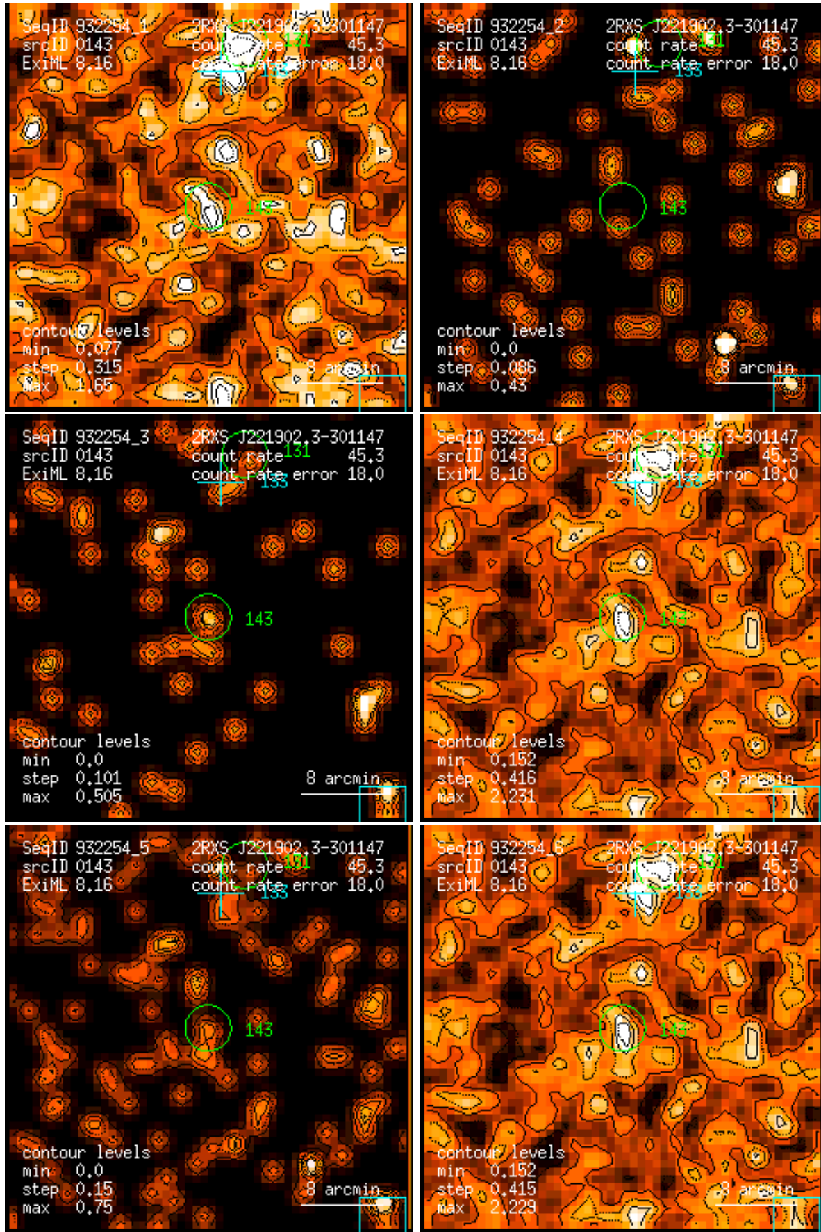
Figure 143: RASS 932254: detection 0143: band rate images, Gaussian filter: (1) PSPC channels 11 – 41, (2) 52 – 90, (3) 91 – 201, (4) 11 – 235, (5) 52 – 201, (6) 11 – 201. Broad band rates in counts/ks. Band rate contour levels in counts/ks/arcmin 2 .
