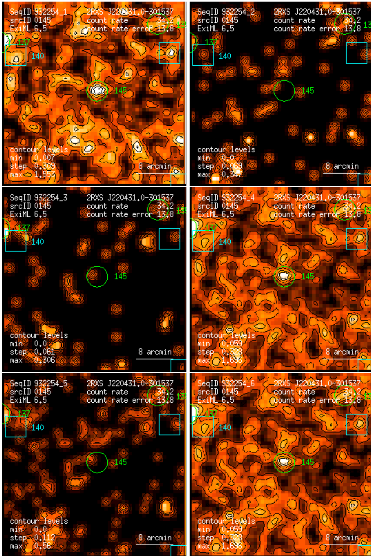
Figure 145: RASS 932254: detection 0145: band rate images, Gaussian filter: (1) PSPC channels 11 – 41, (2) 52 – 90, (3) 91 – 201, (4) 11 – 235, (5) 52 – 201, (6) 11 – 201. Broad band rates in counts/ks. Band rate contour levels in counts/ks/arcmin 2 .
