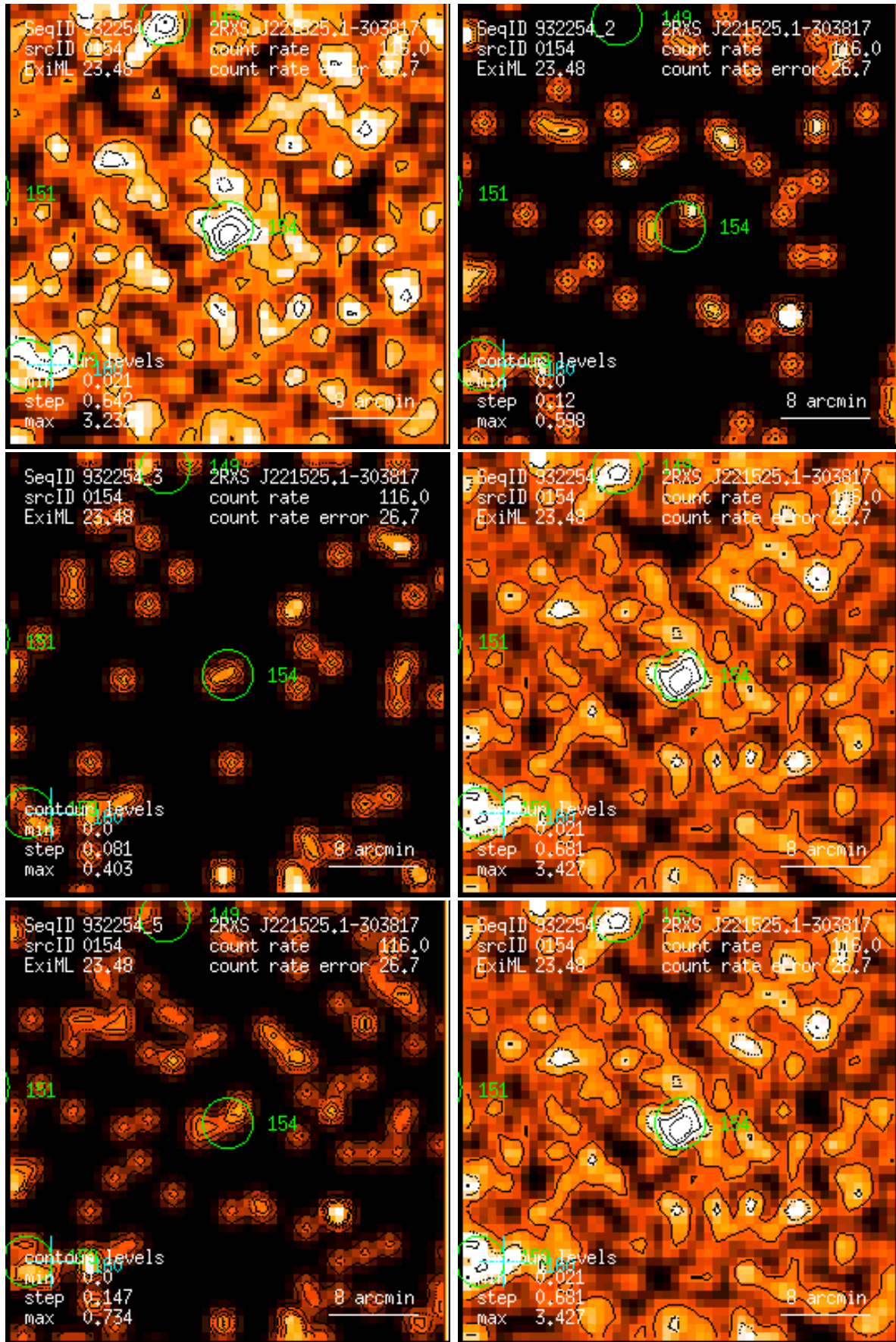
Figure 154: RASS 932254: detection 0154: band rate images, Gaussian filter: (1) PSPC channels 11 – 41, (2) 52 – 90, (3) 91 – 201, (4) 11 – 235, (5) 52 – 201, (6) 11 – 201. Broad band rates in counts/ks. Band rate contour levels in counts/ks/arcmin 2 .
