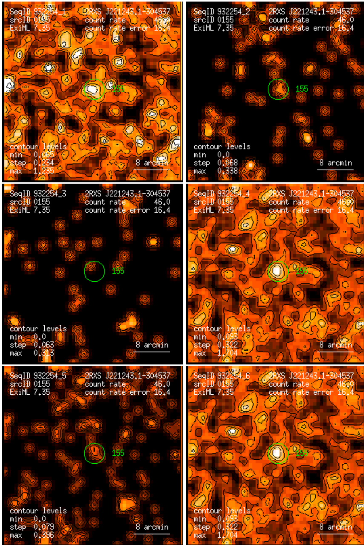
Figure 155: RASS 932254: detection 0155: band rate images, Gaussian filter: (1) PSPC channels 11 – 41, (2) 52 – 90, (3) 91 – 201, (4) 11 – 235, (5) 52 – 201, (6) 11 – 201. Broad band rates in counts/ks. Band rate contour levels in counts/ks/arcmin 2 .
