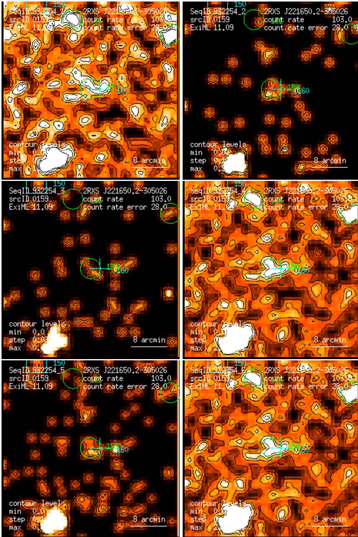
Figure 159: RASS 932254: detection 0159: band rate images, Gaussian filter: (1) PSPC channels 11 – 41, (2) 52 – 90, (3) 91 – 201, (4) 11 – 235, (5) 52 – 201, (6) 11 – 201. Broad band rates in counts/ks. Band rate contour levels in counts/ks/arcmin 2 .
