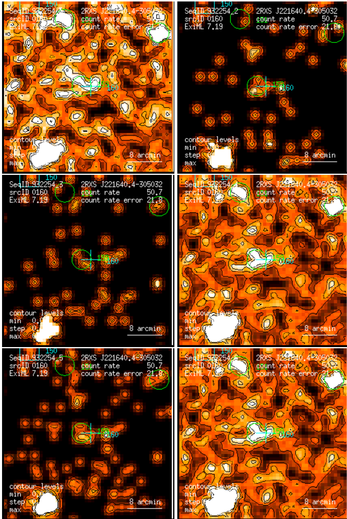
Figure 160: RASS 932254: detection 0160: band rate images, Gaussian filter: (1) PSPC channels 11 – 41, (2) 52 – 90, (3) 91 – 201, (4) 11 – 235, (5) 52 – 201, (6) 11 – 201. Broad band rates in counts/ks. Band rate contour levels in counts/ks/arcmin 2 .
