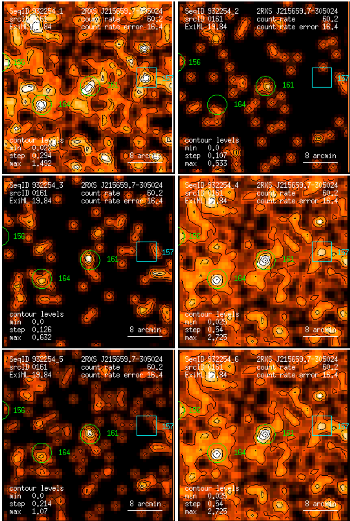
Figure 161: RASS 932254: detection 0161: band rate images, Gaussian filter: (1) PSPC channels 11 – 41, (2) 52 – 90, (3) 91 – 201, (4) 11 – 235, (5) 52 – 201, (6) 11 – 201. Broad band rates in counts/ks. Band rate contour levels in counts/ks/arcmin 2 .
