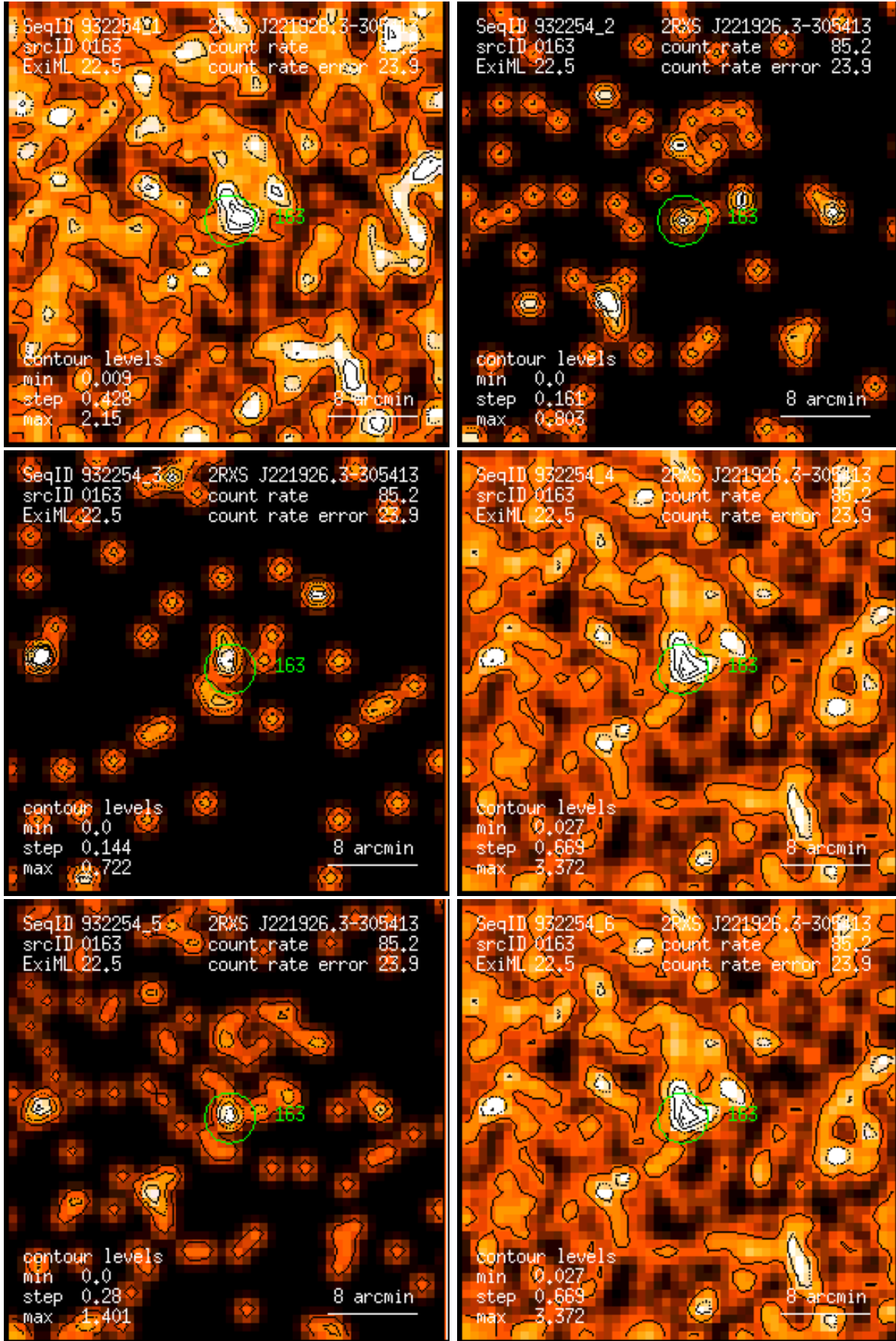
Figure 163: RASS 932254: detection 0163: band rate images, Gaussian filter: (1) PSPC channels 11 – 41, (2) 52 – 90, (3) 91 – 201, (4) 11 – 235, (5) 52 – 201, (6) 11 – 201. Broad band rates in counts/ks. Band rate contour levels in counts/ks/arcmin 2 .
