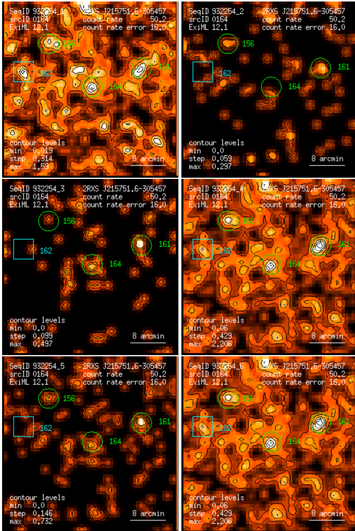
Figure 164: RASS 932254: detection 0164: band rate images, Gaussian filter: (1) PSPC channels 11 – 41, (2) 52 – 90, (3) 91 – 201, (4) 11 – 235, (5) 52 – 201, (6) 11 – 201. Broad band rates in counts/ks. Band rate contour levels in counts/ks/arcmin 2 .
