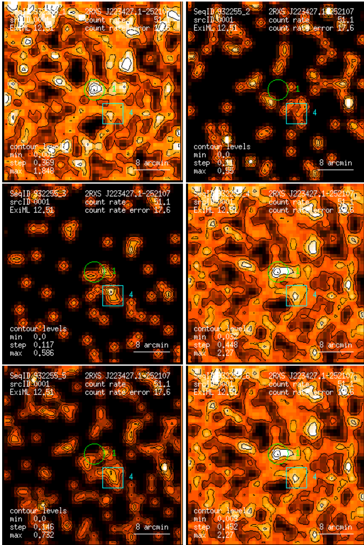
Figure 1: RASS 932255: detection 0001: band rate images, Gaussian filter: (1) PSPC channels 11 – 41, (2) 52 – 90, (3) 91 – 201, (4) 11 – 235, (5) 52 – 201, (6) 11 – 201. Broad band rates in counts/ks. Band rate contour levels in counts/ks/arcmin 2 .
