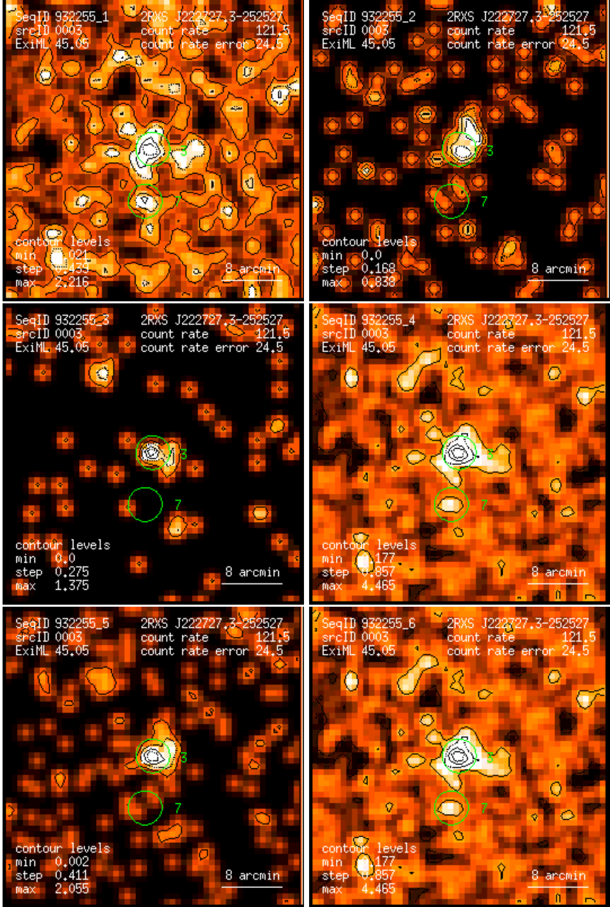
Figure 3: RASS 932255: detection 0003: band rate images, Gaussian filter: (1) PSPC channels 11 – 41, (2) 52 – 90, (3) 91 – 201, (4) 11 – 235, (5) 52 – 201, (6) 11 – 201. Broad band rates in counts/ks. Band rate contour levels in counts/ks/arcmin 2 .
