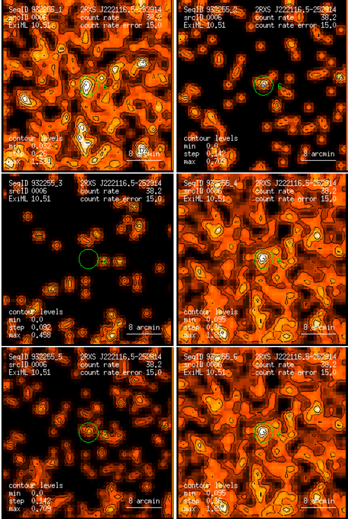
Figure 6: RASS 932255: detection 0006: band rate images, Gaussian filter: (1) PSPC channels 11 – 41, (2) 52 – 90, (3) 91 – 201, (4) 11 – 235, (5) 52 – 201, (6) 11 – 201. Broad band rates in counts/ks. Band rate contour levels in counts/ks/arcmin 2 .
