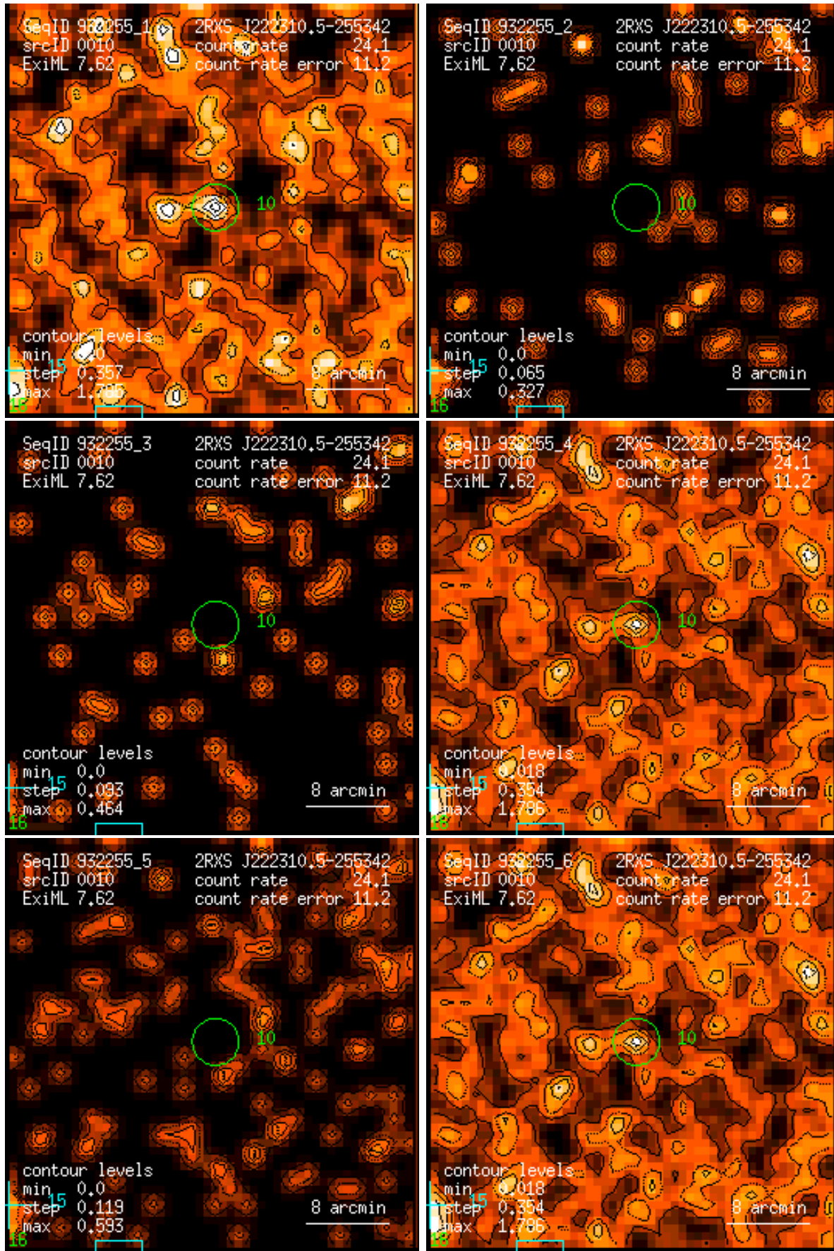
Figure 10: RASS 932255: detection 0010: band rate images, Gaussian filter: (1) PSPC channels 11 – 41, (2) 52 – 90, (3) 91 – 201, (4) 11 – 235, (5) 52 – 201, (6) 11 – 201. Broad band rates in counts/ks. Band rate contour levels in counts/ks/arcmin 2 .
