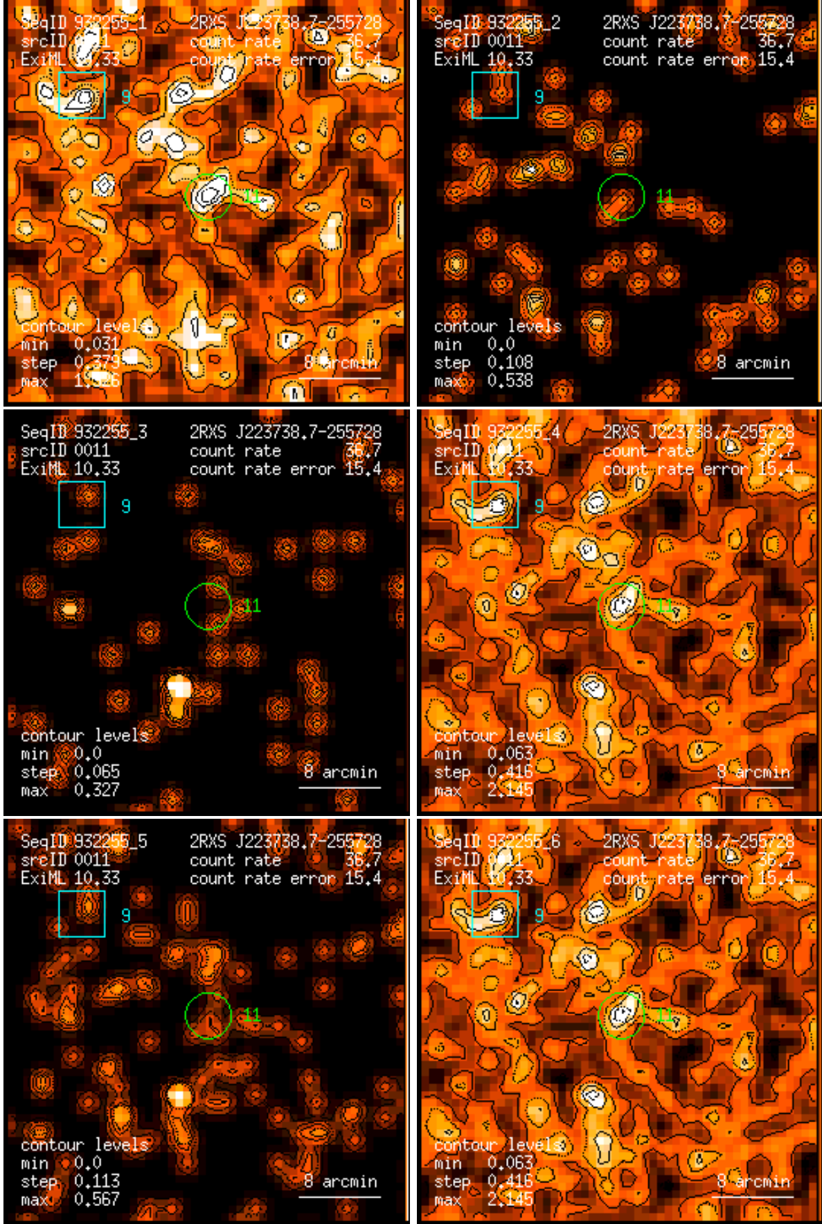
Figure 11: RASS 932255: detection 0011: band rate images, Gaussian filter: (1) PSPC channels 11 – 41, (2) 52 – 90, (3) 91 – 201, (4) 11 – 235, (5) 52 – 201, (6) 11 – 201. Broad band rates in counts/ks. Band rate contour levels in counts/ks/arcmin 2 .
