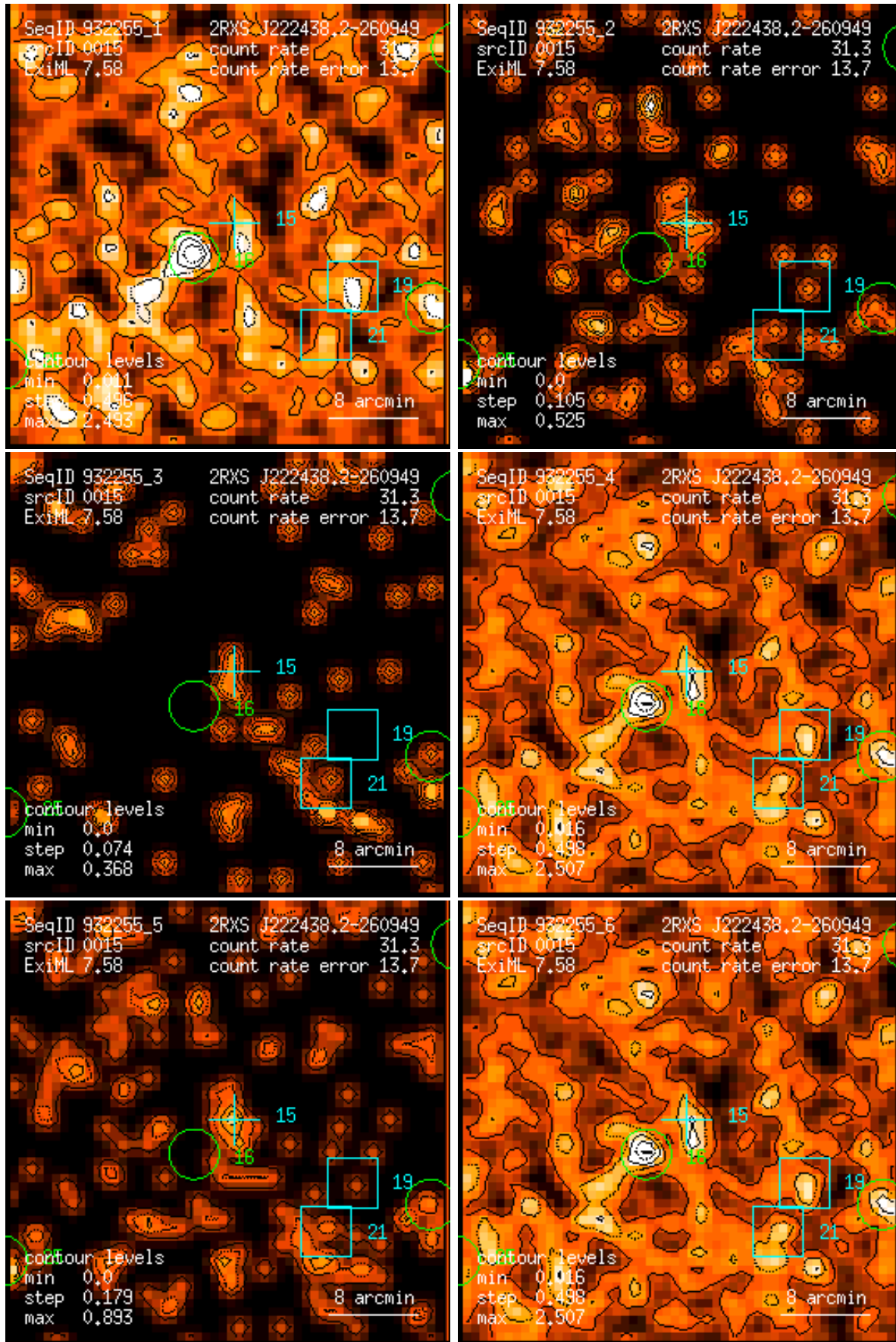
Figure 15: RASS 932255: detection 0015: band rate images, Gaussian filter: (1) PSPC channels 11 – 41, (2) 52 – 90, (3) 91 – 201, (4) 11 – 235, (5) 52 – 201, (6) 11 – 201. Broad band rates in counts/ks. Band rate contour levels in counts/ks/arcmin 2 .
