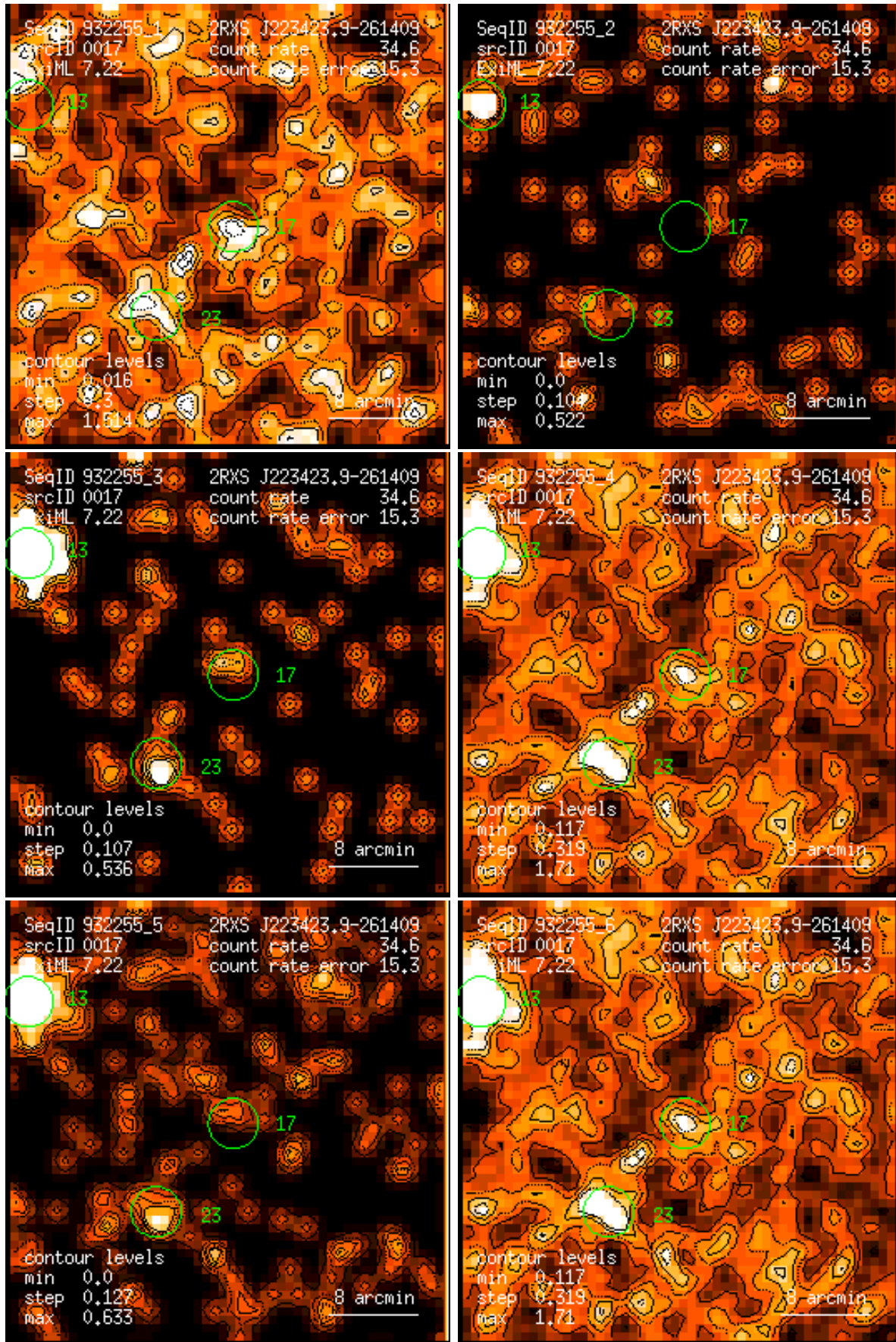
Figure 17: RASS 932255: detection 0017: band rate images, Gaussian filter: (1) PSPC channels 11 – 41, (2) 52 – 90, (3) 91 – 201, (4) 11 – 235, (5) 52 – 201, (6) 11 – 201. Broad band rates in counts/ks. Band rate contour levels in counts/ks/arcmin 2 .
