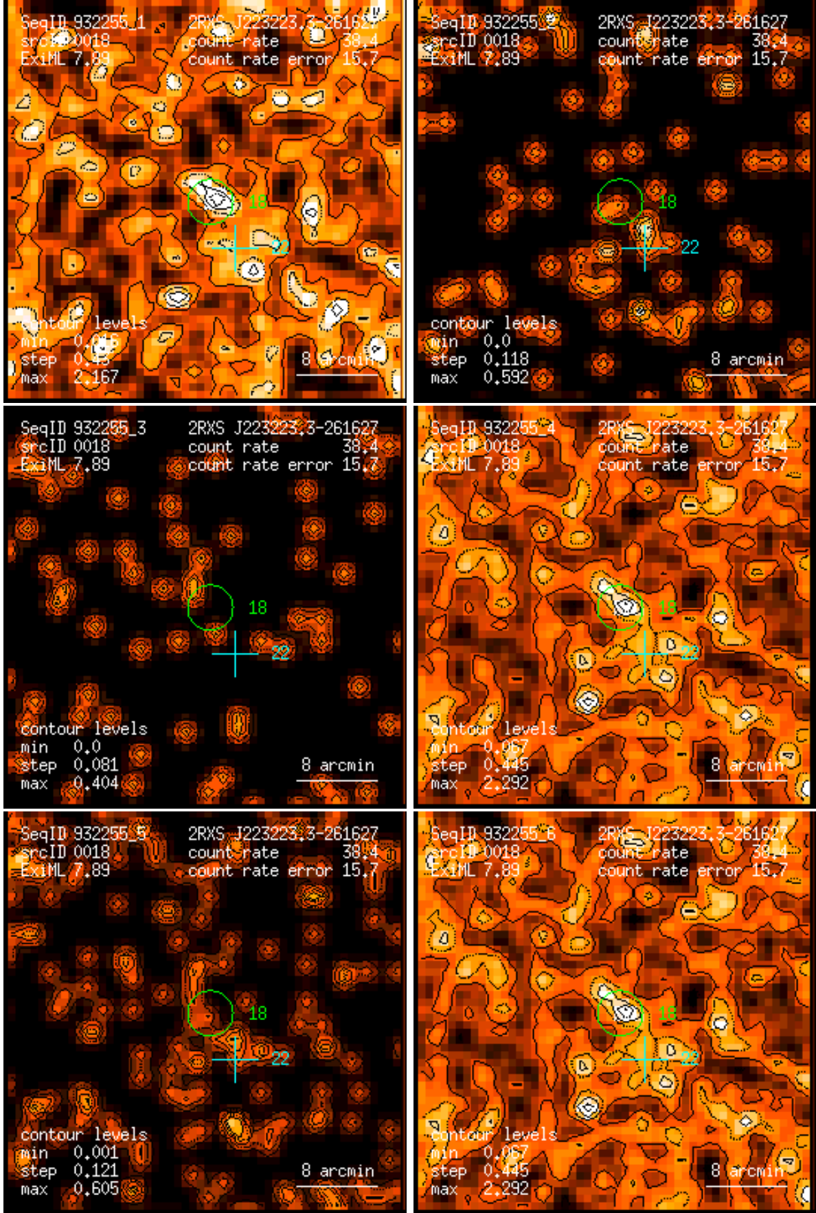
Figure 18: RASS 932255: detection 0018: band rate images, Gaussian filter: (1) PSPC channels 11 – 41, (2) 52 – 90, (3) 91 – 201, (4) 11 – 235, (5) 52 – 201, (6) 11 – 201. Broad band rates in counts/ks. Band rate contour levels in counts/ks/arcmin 2 .
