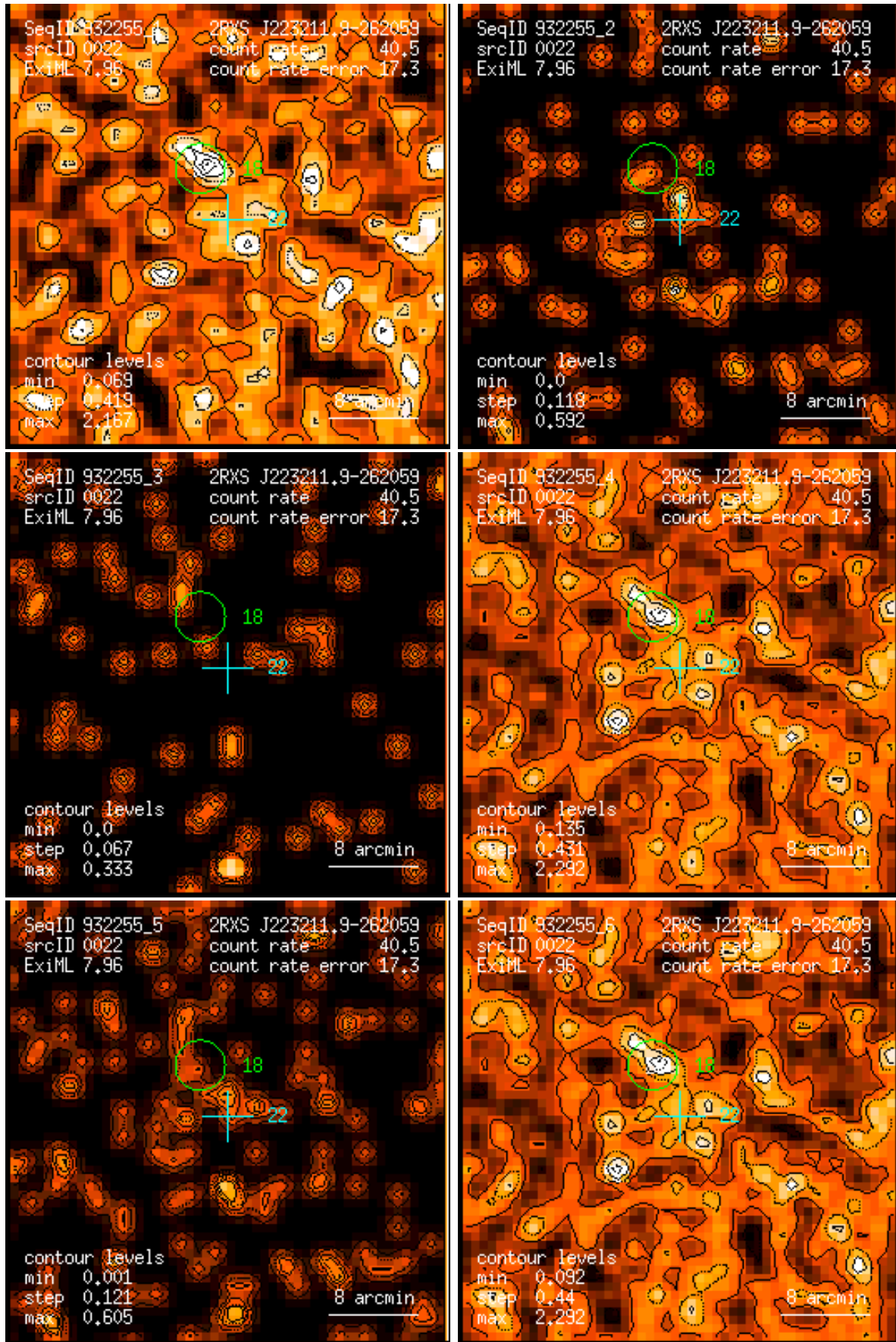
Figure 22: RASS 932255: detection 0022: band rate images, Gaussian filter: (1) PSPC channels 11 – 41, (2) 52 – 90, (3) 91 – 201, (4) 11 – 235, (5) 52 – 201, (6) 11 – 201. Broad band rates in counts/ks. Band rate contour levels in counts/ks/arcmin 2 .
