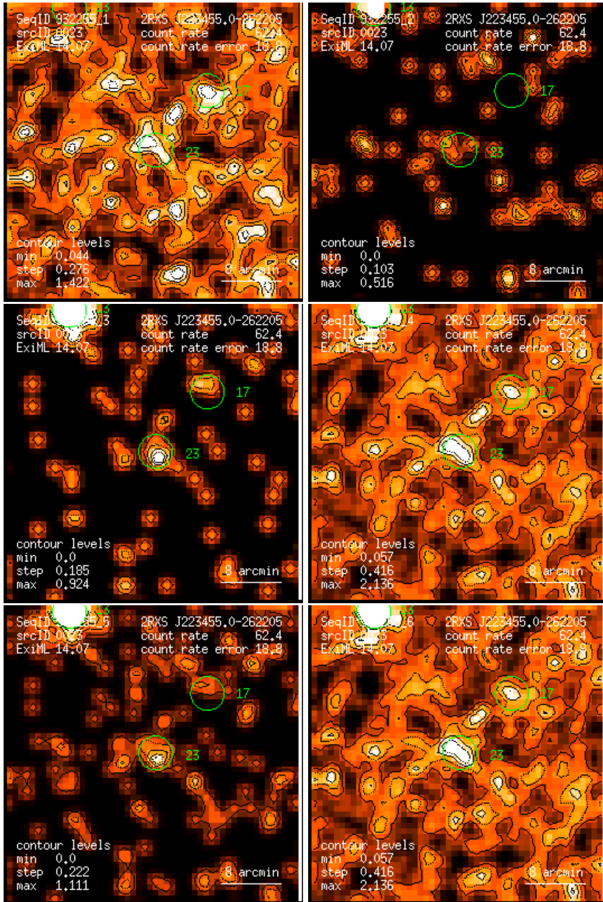
Figure 23: RASS 932255: detection 0023: band rate images, Gaussian filter: (1) PSPC channels 11 – 41, (2) 52 – 90, (3) 91 – 201, (4) 11 – 235, (5) 52 – 201, (6) 11 – 201. Broad band rates in counts/ks. Band rate contour levels in counts/ks/arcmin 2 .
