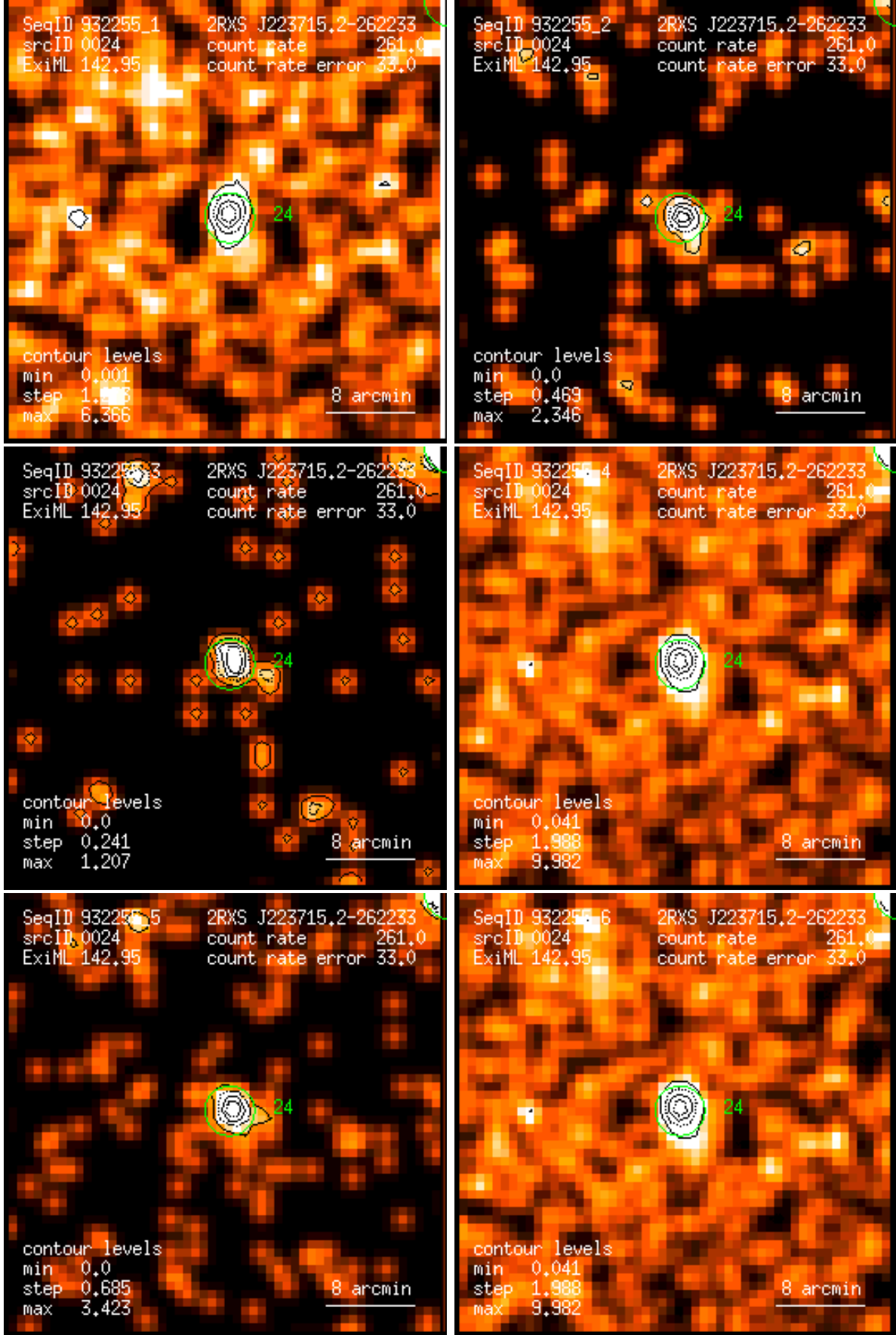
Figure 24: RASS 932255: detection 0024: band rate images, Gaussian filter: (1) PSPC channels 11 – 41, (2) 52 – 90, (3) 91 – 201, (4) 11 – 235, (5) 52 – 201, (6) 11 – 201. Broad band rates in counts/ks. Band rate contour levels in counts/ks/arcmin 2 .
