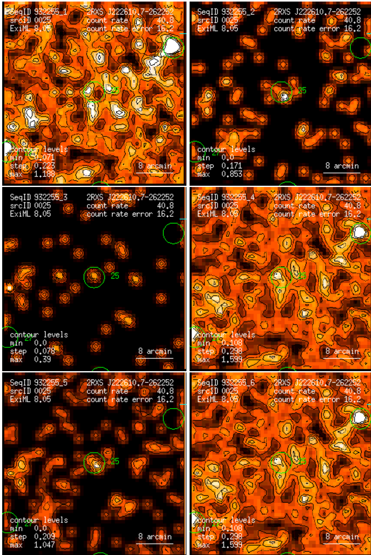
Figure 25: RASS 932255: detection 0025: band rate images, Gaussian filter: (1) PSPC channels 11 – 41, (2) 52 – 90, (3) 91 – 201, (4) 11 – 235, (5) 52 – 201, (6) 11 – 201. Broad band rates in counts/ks. Band rate contour levels in counts/ks/arcmin 2 .
