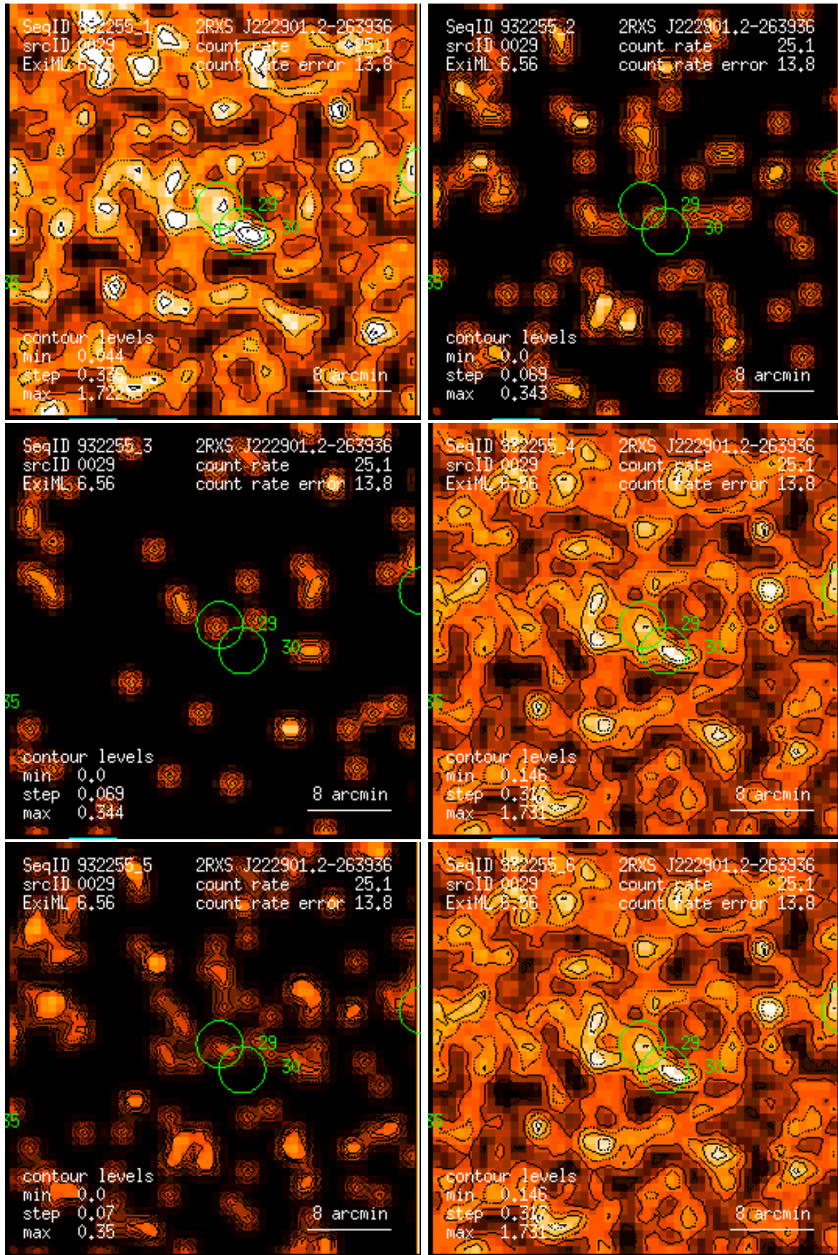
Figure 29: RASS 932255: detection 0029: band rate images, Gaussian filter: (1) PSPC channels 11 – 41, (2) 52 – 90, (3) 91 – 201, (4) 11 – 235, (5) 52 – 201, (6) 11 – 201. Broad band rates in counts/ks. Band rate contour levels in counts/ks/arcmin 2 .
