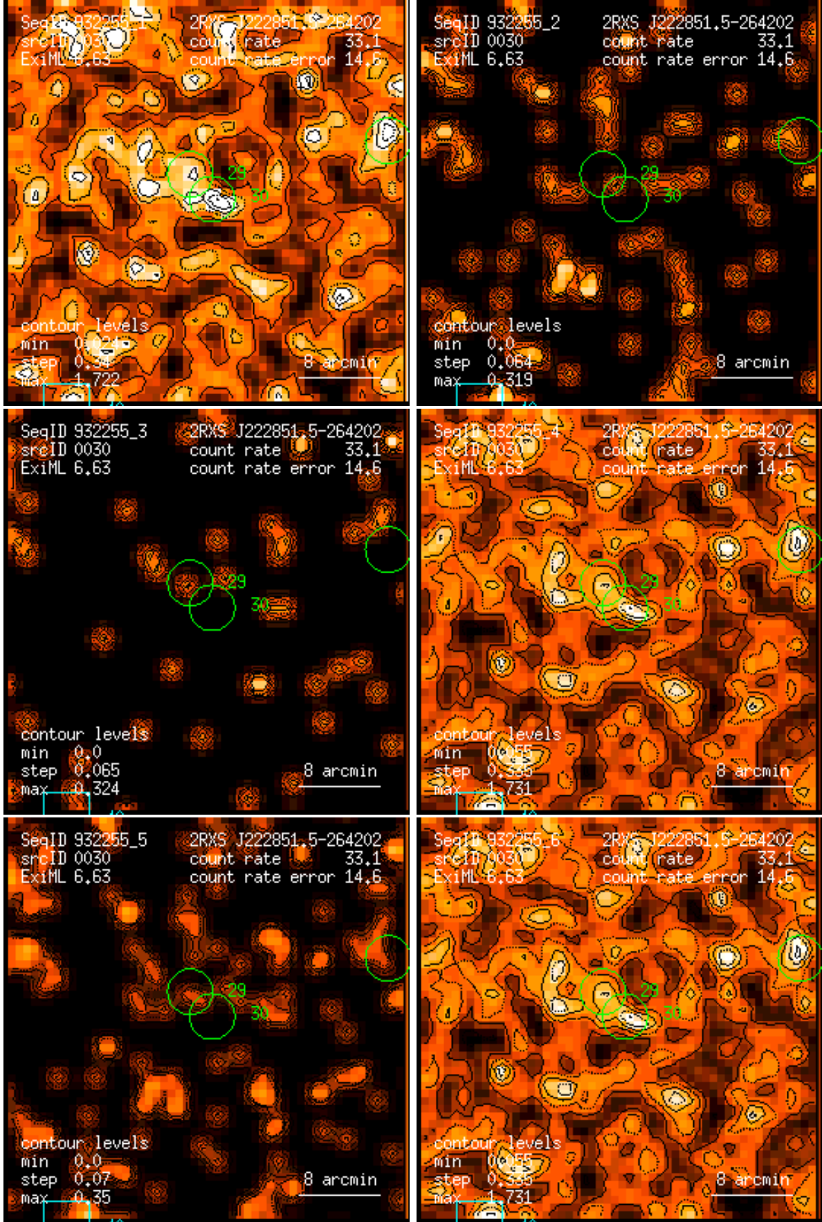
Figure 30: RASS 932255: detection 0030: band rate images, Gaussian filter: (1) PSPC channels 11 – 41, (2) 52 – 90, (3) 91 – 201, (4) 11 – 235, (5) 52 – 201, (6) 11 – 201. Broad band rates in counts/ks. Band rate contour levels in counts/ks/arcmin 2 .
